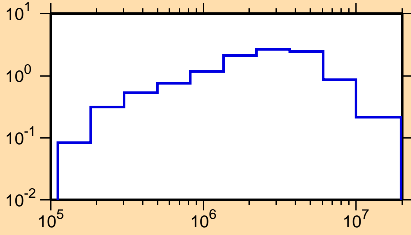
\sigma vs. E for ^{226}\text{Po}(n,\text{inel.})
