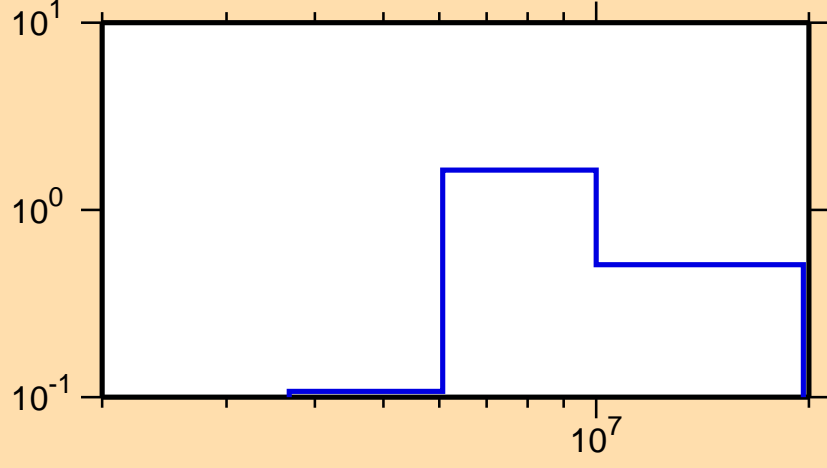
\sigma vs. E for ^{226}\text{Po}(n,2n)
