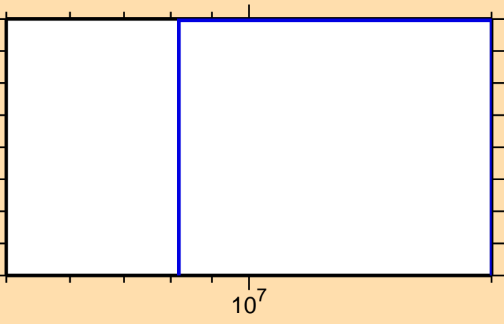
\sigma vs. E for ^{226}\text{Po}(n,p)
