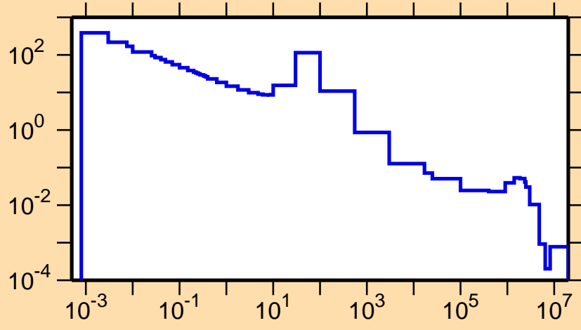
\sigma vs. E for ^{226}\text{Po}(n,\gamma)
