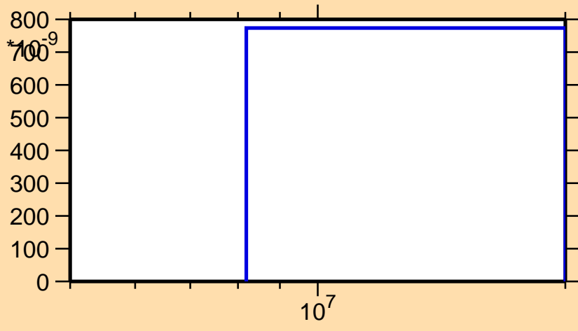
\sigma vs. E for ^{226}\text{Po}(n,d)
