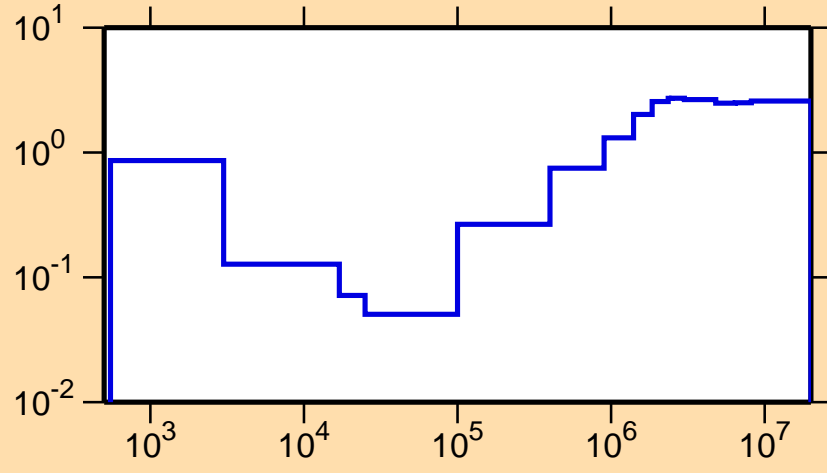
\sigma vs. E for ^{226}\text{Po}(n,\text{nonel.})
