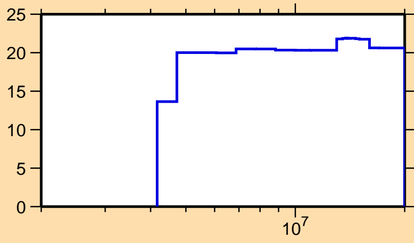
\Delta\sigma/\sigma vs. E for ^{227}\text{Po}(n,\text{nonel.})
