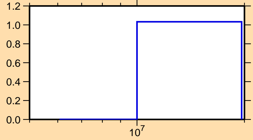
\Delta\sigma/\sigma vs. E for ^{227}\text{Po}(n,f)
