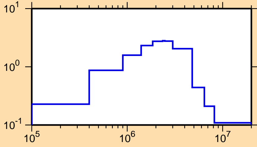
\sigma vs. E for ^{227}\text{Po}(n,\text{inel.})
