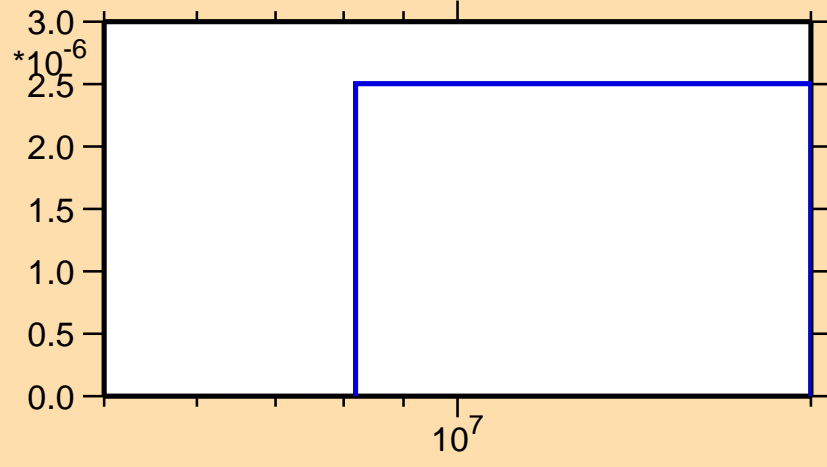
\sigma vs. E for ^{227}\text{Po}(n,d)
