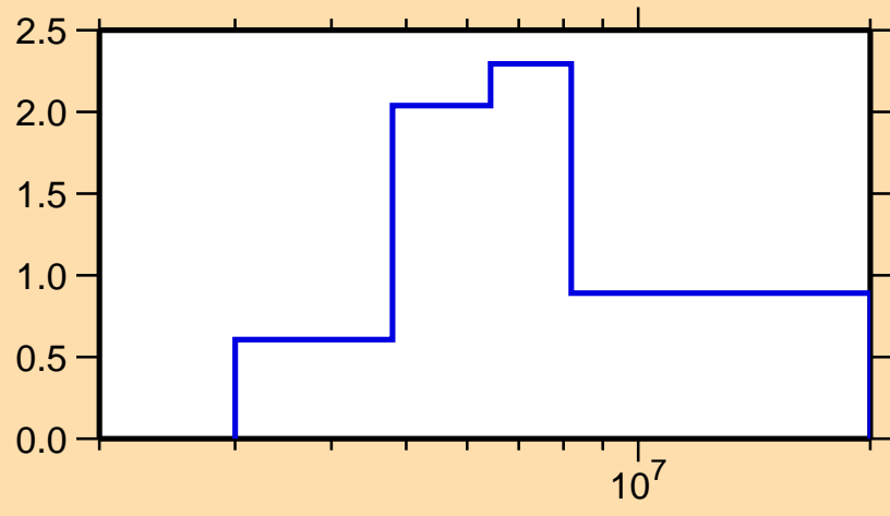
\sigma vs. E for ^{227}\text{Po}(n,2n)
