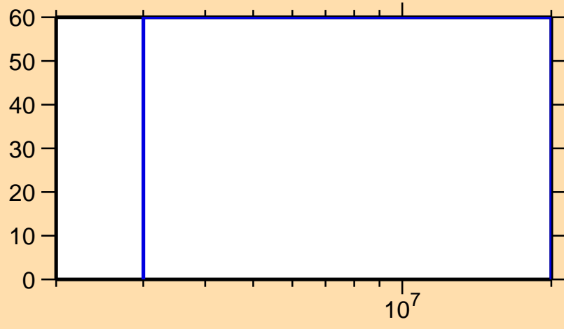
\Delta\sigma/\sigma vs. E for ^{227}\text{Po}(n,2n)
