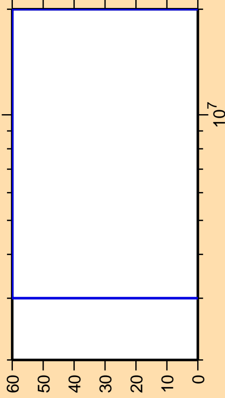
\Delta\sigma/\sigma vs. E for ^{227}\text{Po}(n,n\text{cont.})
