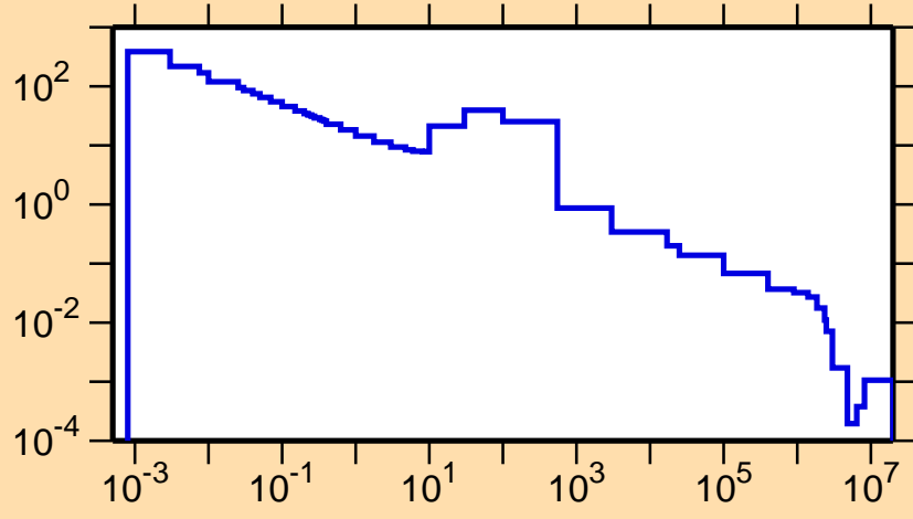
\sigma vs. E for ^{227}\text{Po}(n,\gamma)
