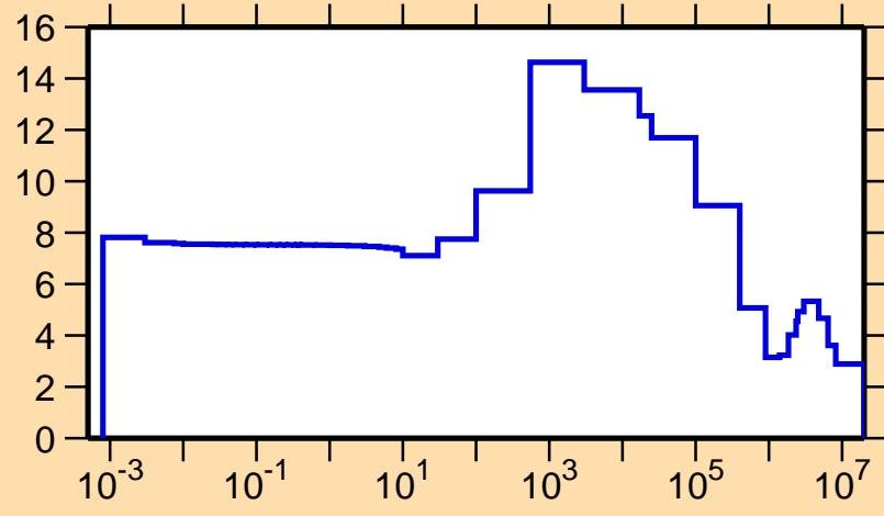
\sigma vs. E for ^{227}\text{Po}(n,\text{el.})
