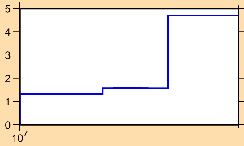
\Delta\sigma/\sigma vs. E for ^{124}\text{Pr}(n,\text{tot.})
