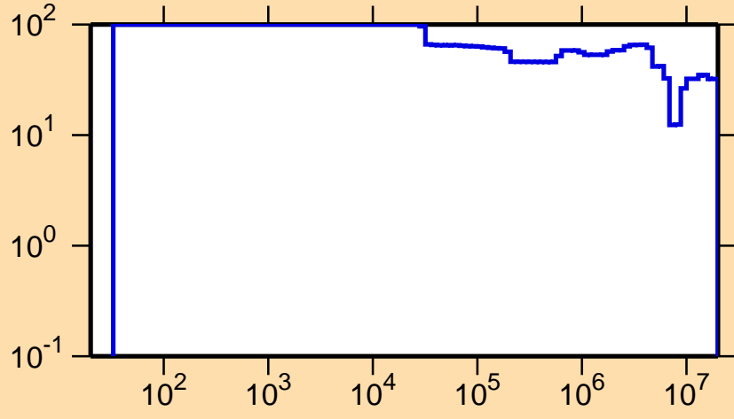
\Delta\sigma/\sigma vs. E for ^{124}\text{Pr}(n,p)
