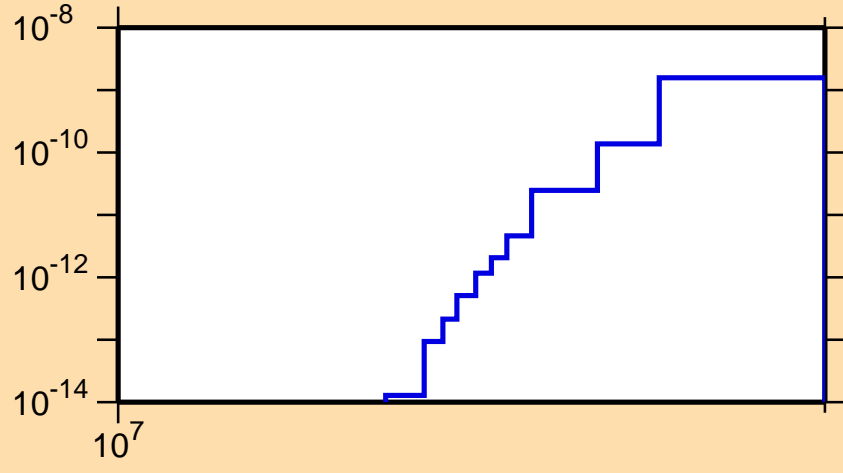
\sigma vs. E for ^{124}\text{Pr}(n,2n\alpha)
