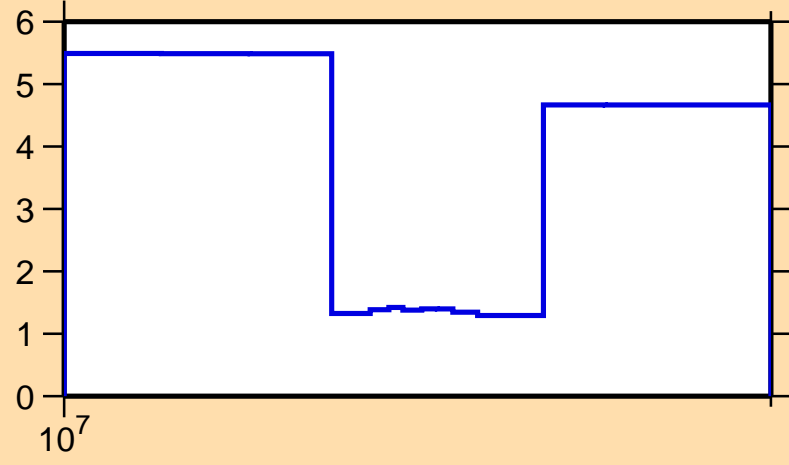
\Delta\sigma/\sigma vs. E for ^{124}\text{Pr}(n,\text{el.})
