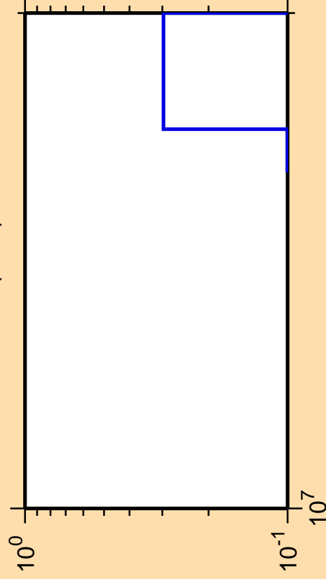
\Delta\sigma/\sigma vs. E for ^{124}\text{Pr}(n,nt)
