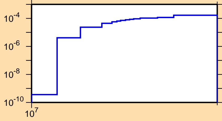
\sigma vs. E for ^{124}\text{Pr}(n,2n)
