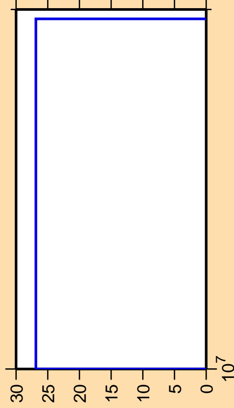
\Delta\sigma/\sigma vs. E for ^{124}\text{Pr}(n,n\text{cont.})
