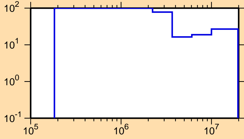
\Delta\sigma/\sigma vs. E for ^{124}\text{Pr}(n,n\text{cont.})
