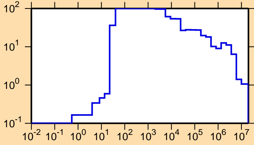
\Delta\sigma/\sigma vs. E for ^{124}\text{Pr}(n,\text{tot.})
