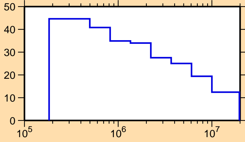
\Delta\sigma/\sigma vs. E for ^{124}\text{Pr}(n,n_1)
