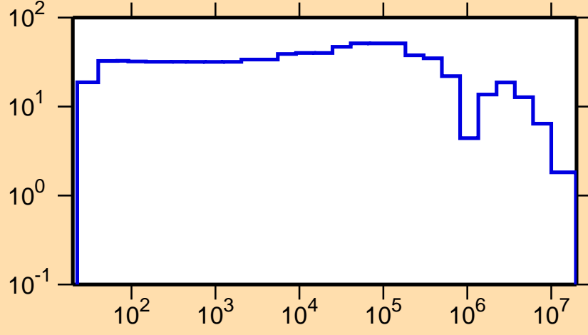
\Delta\sigma/\sigma vs. E for ^{124}\text{Pr}(n,\text{el.})
