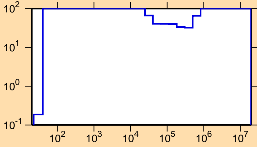
\Delta\sigma/\sigma vs. E for ^{124}\text{Pr}(n,\gamma)
