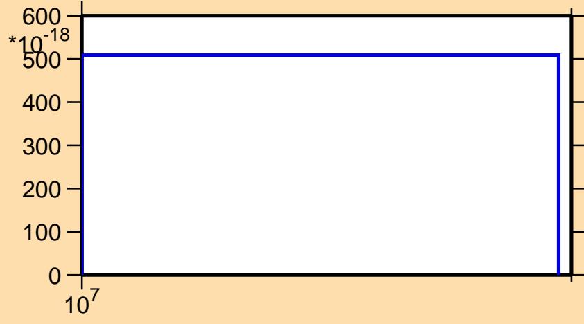
\sigma vs. E for ^{124}\text{Pr}(n,nt)
