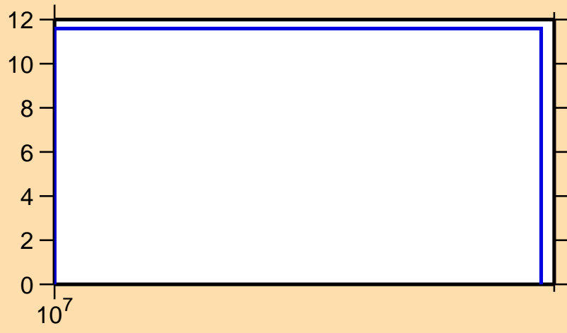
\Delta\sigma/\sigma vs. E for ^{124}\text{Pr}(n,\text{inel.})
