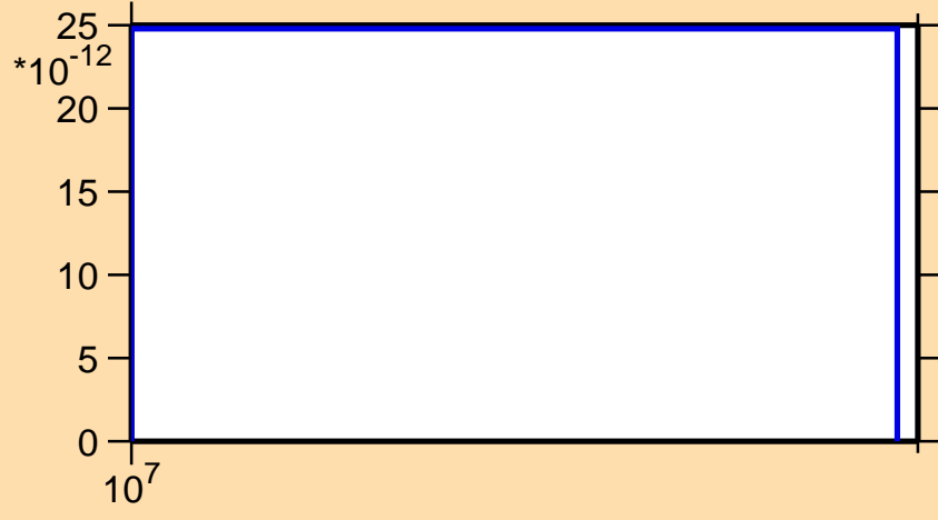
\sigma vs. E for ^{124}\text{Pr}(n,2n\alpha)
