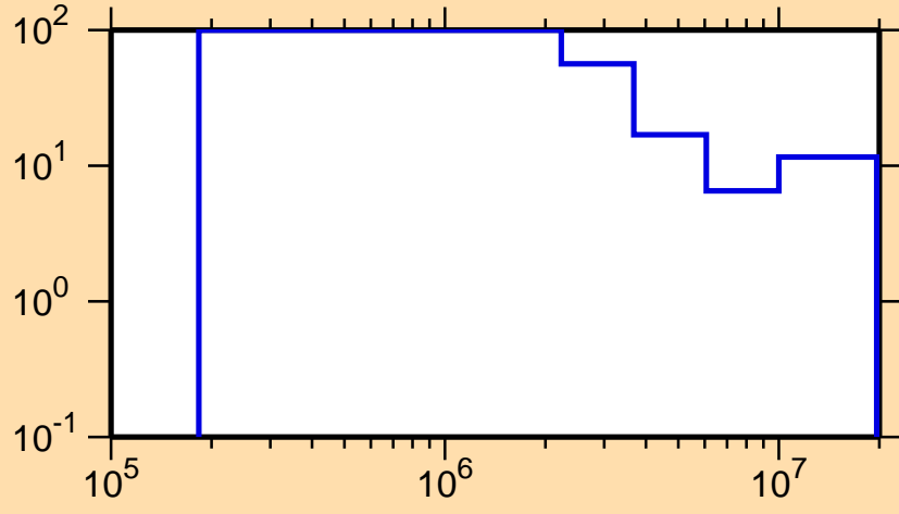
\Delta\sigma/\sigma vs. E for ^{124}\text{Pr}(n,\text{inel.})
