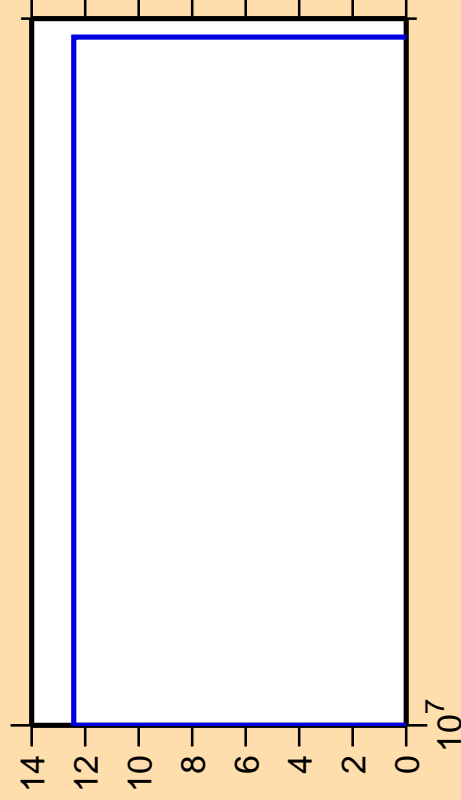
\Delta\sigma/\sigma vs. E for ^{124}\text{Pr}(n,n_1)
