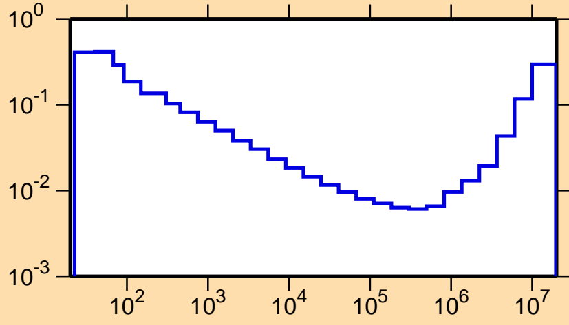
\sigma vs. E for ^{124}\text{Pr}(n,p\alpha)
