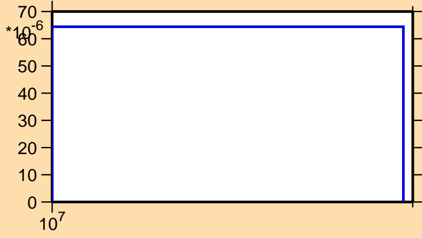
\sigma vs. E for ^{124}\text{Pr}(n,2n)
