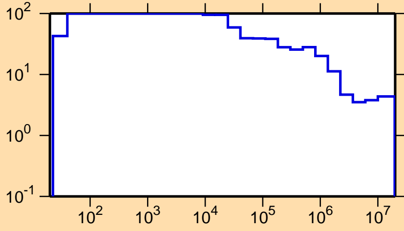
\Delta\sigma/\sigma vs. E for ^{124}\text{Pr}(n,\text{nonel.})
