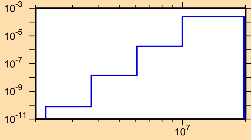
\sigma vs. E for ^{124}\text{Pr}(n,n\alpha)
