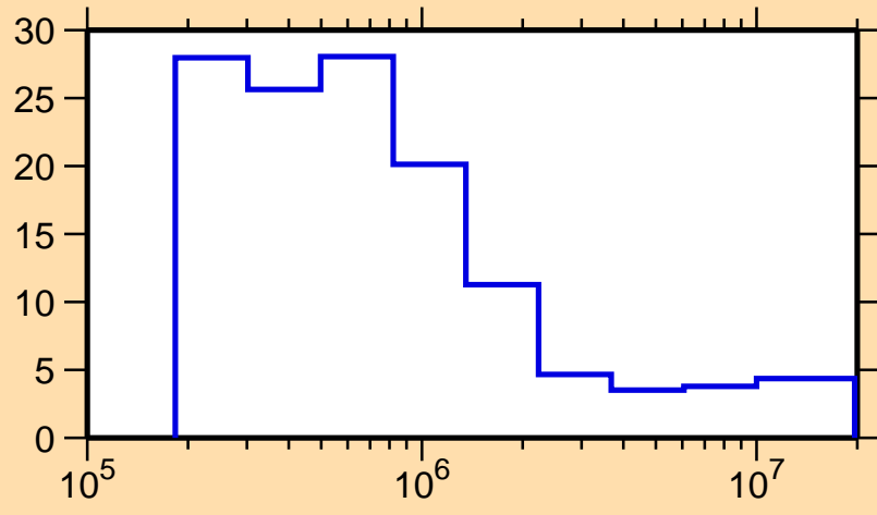
\Delta\sigma/\sigma vs. E for ^{124}\text{Pr}(n, \text{nonel.})
