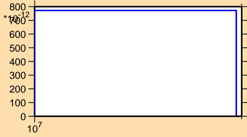
\sigma vs. E for ^{124}\text{Pr}(\text{mt } 34)
