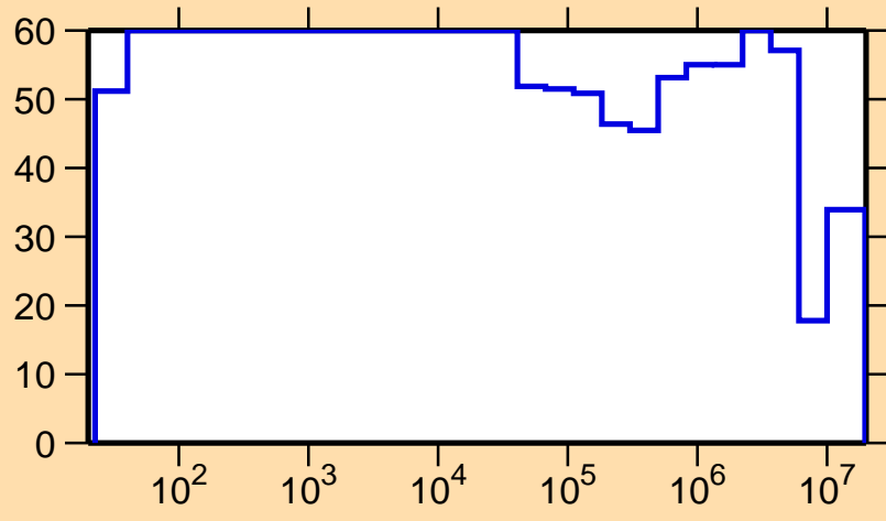
\Delta\sigma/\sigma vs. E for ^{124}\text{Pr}(n,p)
