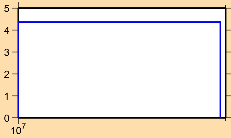
\Delta\sigma/\sigma vs. E for ^{124}\text{Pr}(n,\text{nonel.})
