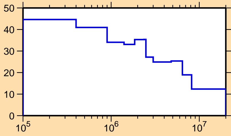
\Delta\sigma/\sigma vs. E for ^{124}\text{Pr}(n,n_1)
