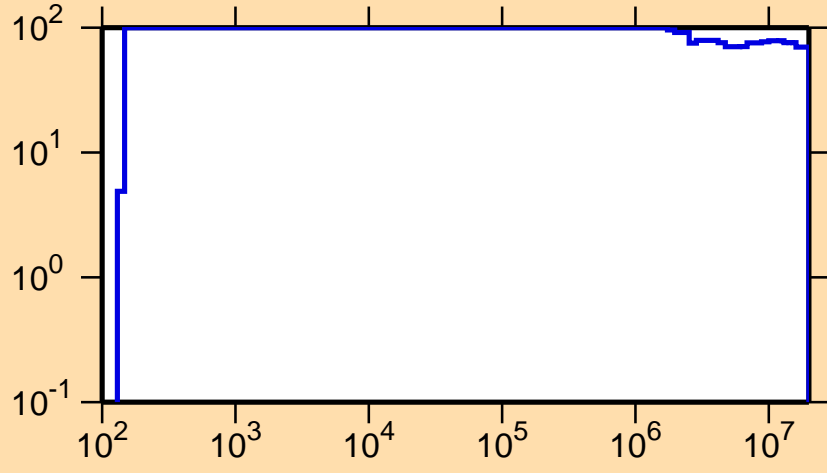
\Delta\sigma/\sigma vs. E for ^{125}\text{Pr}(n,\gamma)
