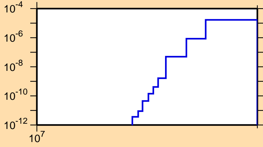
\sigma vs. E for ^{125}\text{Pr}(n,\text{pt})
