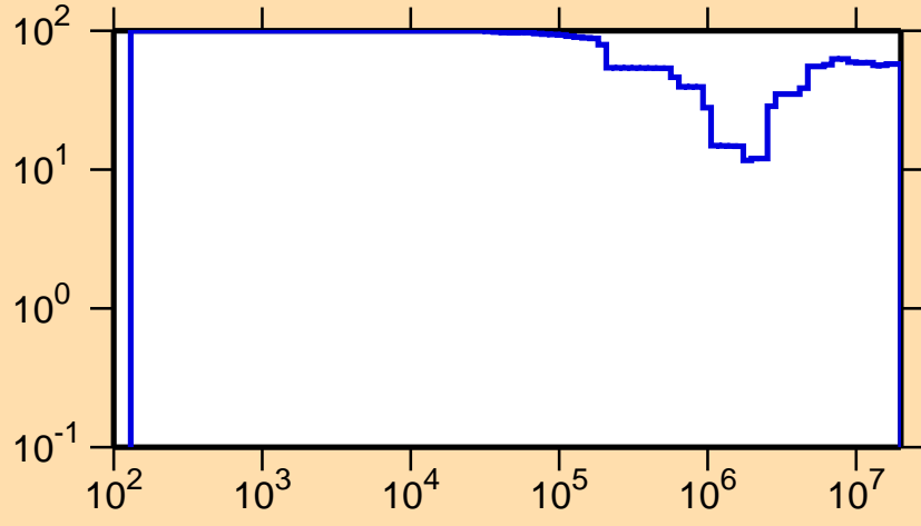
\Delta\sigma/\sigma vs. E for ^{125}\text{Pr}(n,p)
