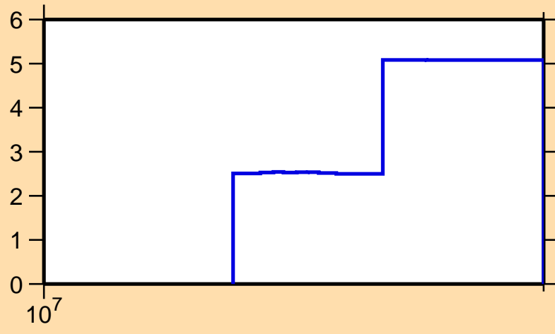
\Delta\sigma/\sigma vs. E for ^{125}\text{Pr}(n,\text{tot.})
