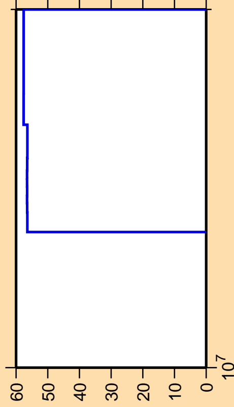
\Delta\sigma/\sigma vs. E for ^{125}\text{Pr}(n,p)
