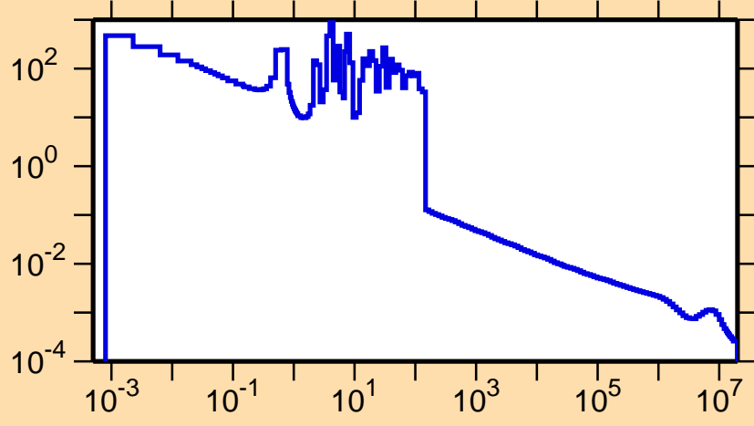
\sigma vs. E for ^{125}\text{Pr}(n,\gamma)
