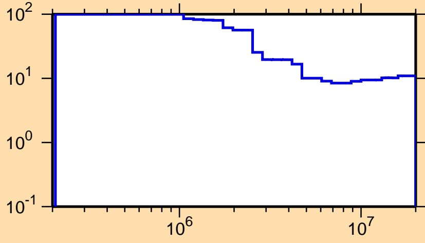
\Delta\sigma/\sigma vs. E for ^{125}\text{Pr}(n,\text{inel.})
