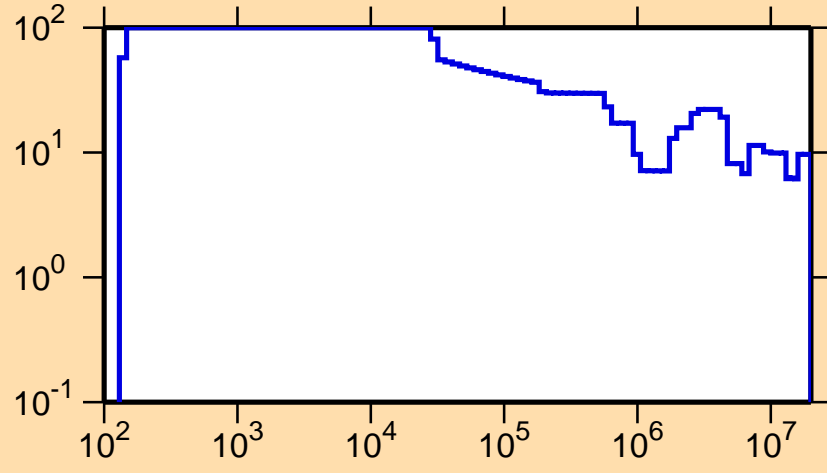
\Delta\sigma/\sigma vs. E for ^{125}\text{Pr}(n,\text{el.})
