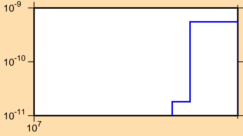
\sigma vs. E for ^{125}\text{Pr}(\text{mt } 34)
