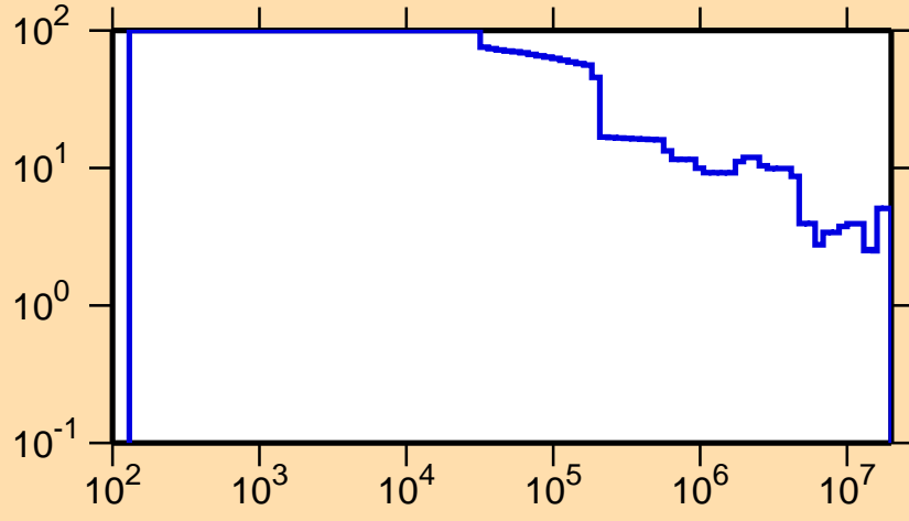
\Delta\sigma/\sigma vs. E for ^{125}\text{Pr}(n,\text{tot.})
