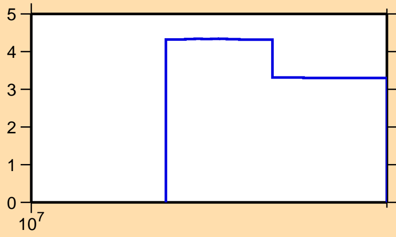
\Delta\sigma/\sigma vs. E for ^{125}\text{Pr}(n,\text{nonel.})
