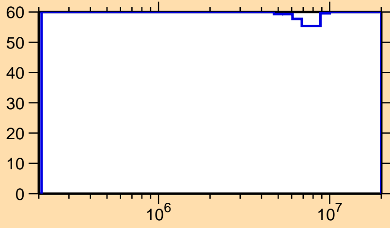
\Delta\sigma/\sigma vs. E for ^{125}\text{Pr}(n,n\text{cont.})
