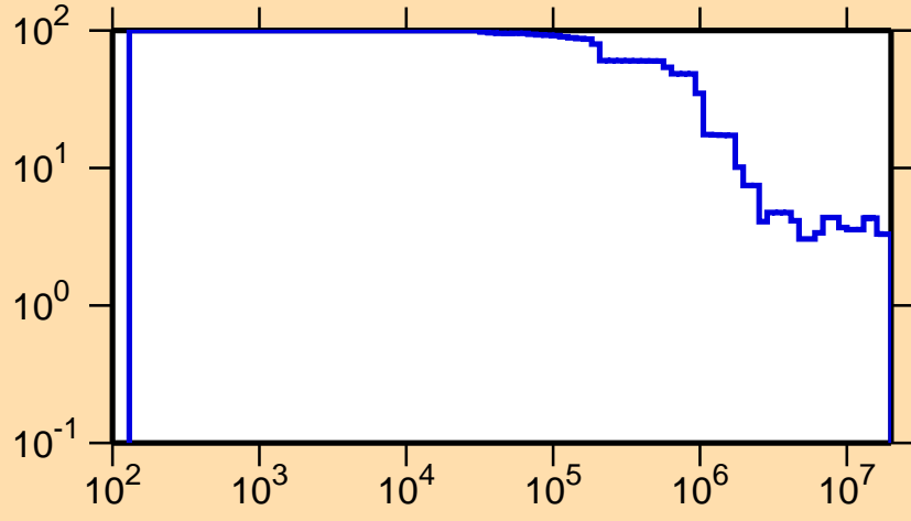
\Delta\sigma/\sigma vs. E for ^{125}\text{Pr}(n,\text{nonel.})
