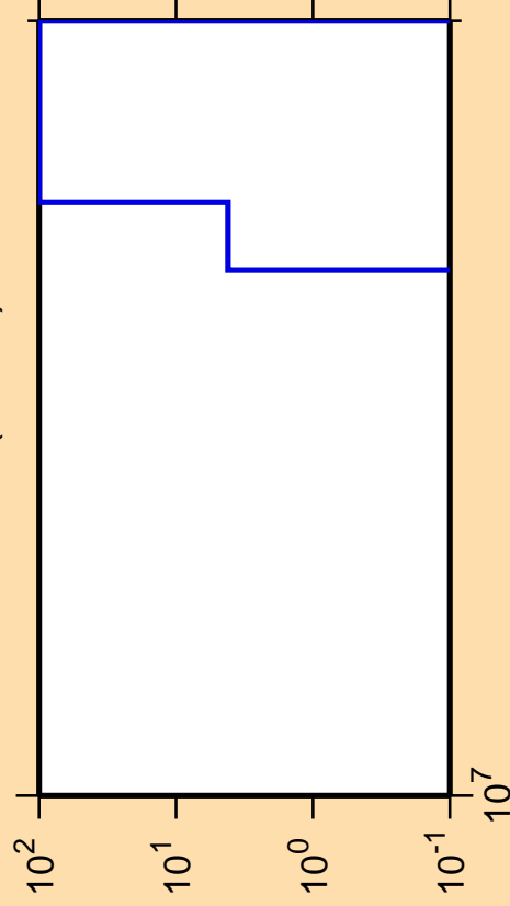
\Delta\sigma/\sigma vs. E for ^{125}\text{Pr}(n,2n\alpha)
