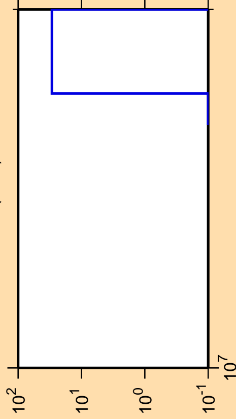
\Delta\sigma/\sigma vs. E for ^{125}\text{Pr}(n,nt)
