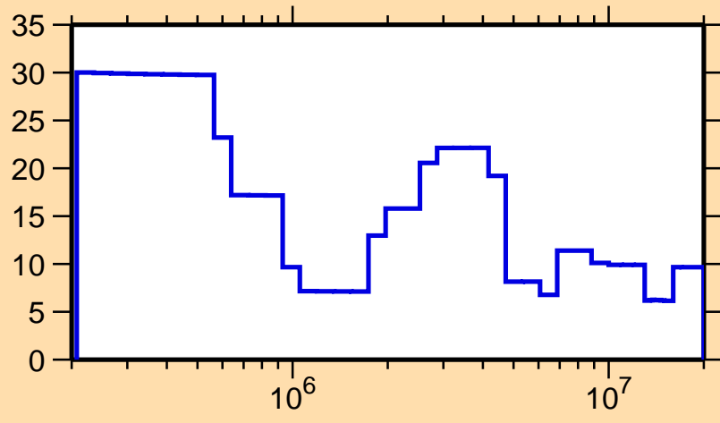
\Delta\sigma/\sigma vs. E for ^{125}\text{Pr}(n,\text{el.})
