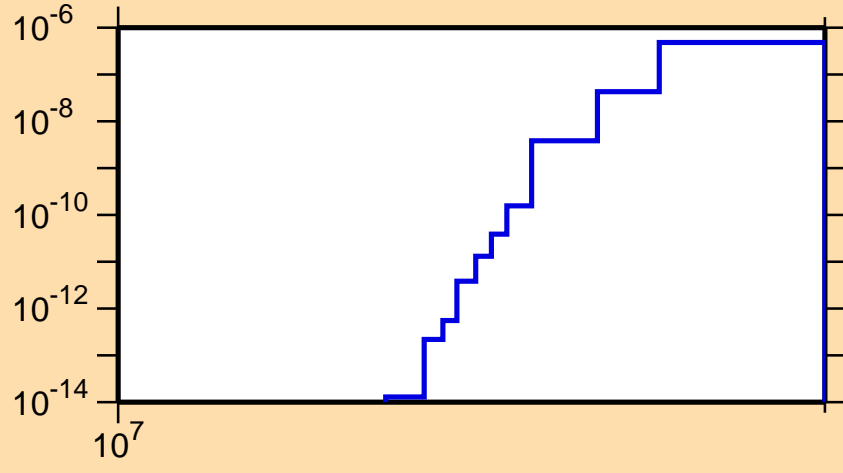
\sigma vs. E for ^{125}\text{Pr}(n,\text{nd})
