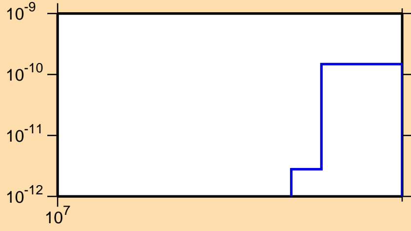
\sigma vs. E for ^{125}\text{Pr}(n,2n\alpha)
