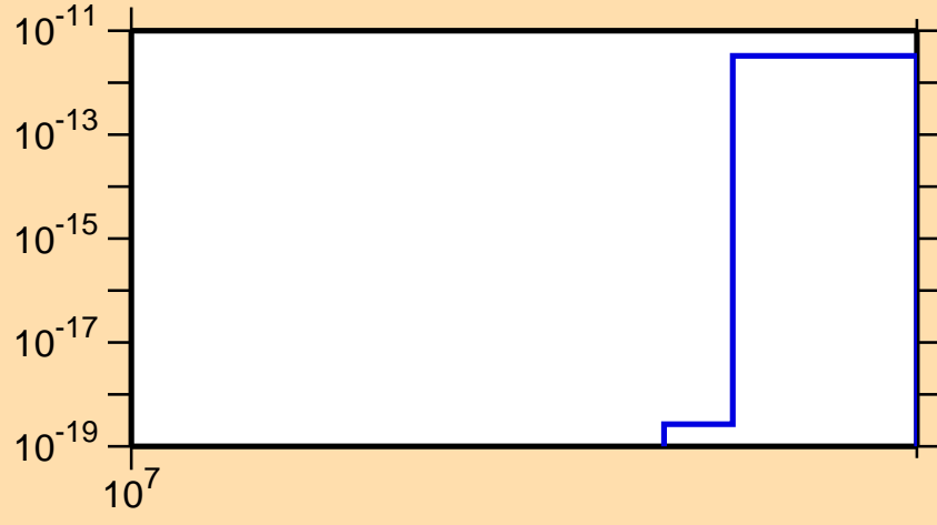
\sigma vs. E for ^{125}\text{Pr}(n,nt)
