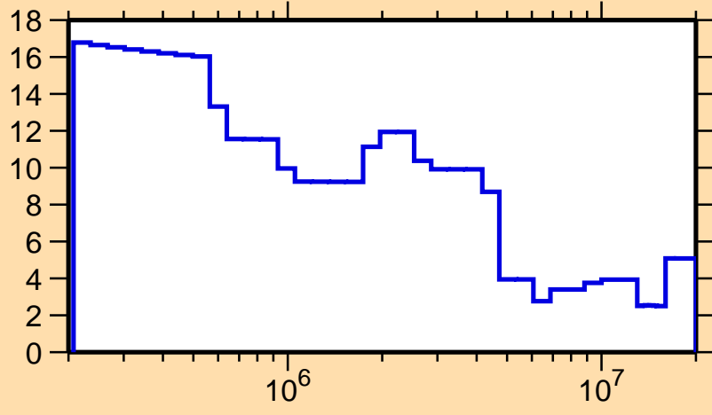
\Delta\sigma/\sigma vs. E for ^{125}\text{Pr}(n,\text{tot.})
