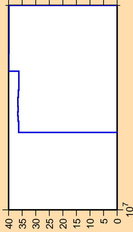
\Delta\sigma/\sigma vs. E for ^{125}\text{Pr}(n,n_1)
