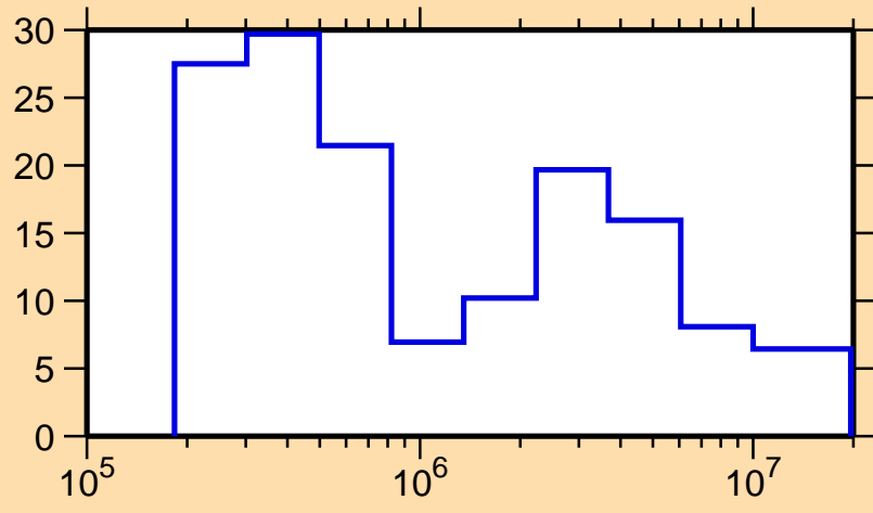
\Delta\sigma/\sigma vs. E for ^{125}\text{Pr}(n, el.)
