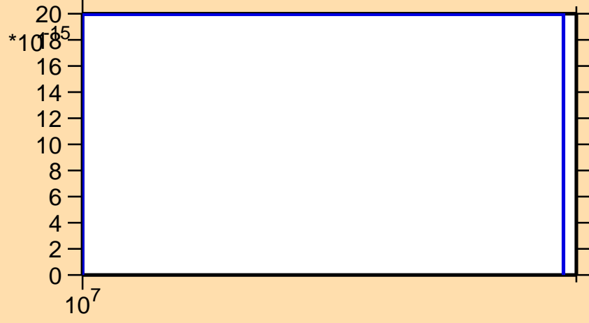
\sigma vs. E for ^{125}\text{Pr}(n,nt)
