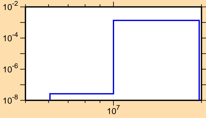
\sigma vs. E for ^{125}\text{Pr}(n,\text{pd})
