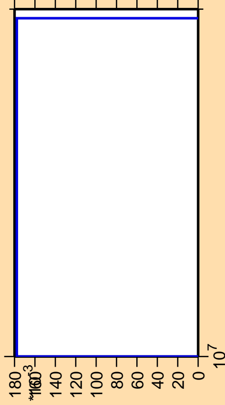
\Delta\sigma/\sigma vs. E for ^{125}\text{Pr}(n,nt)
