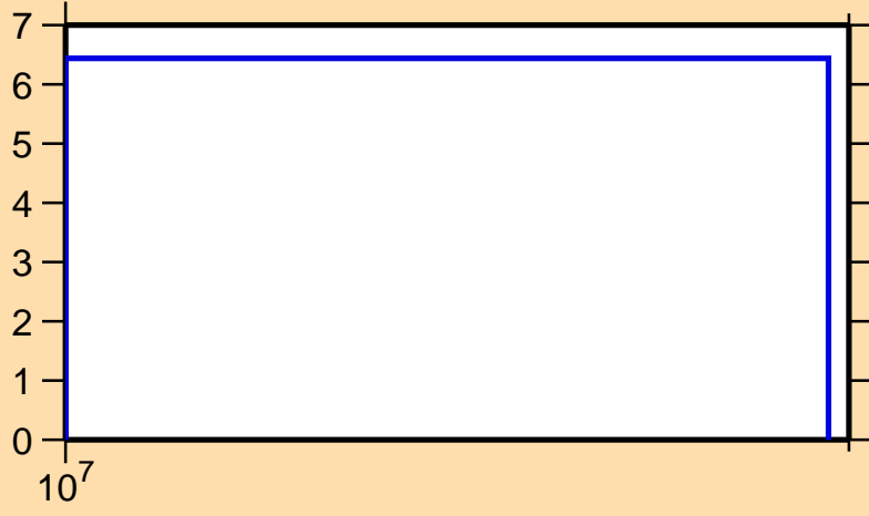
\Delta\sigma/\sigma vs. E for ^{125}\text{Pr}(n,\text{el.})
