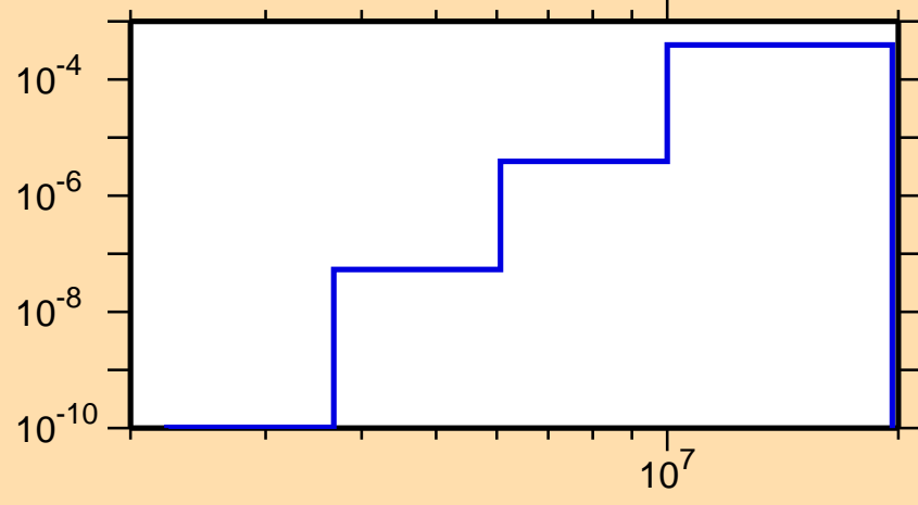
\sigma vs. E for ^{125}\text{Pr}(n,n\alpha)
