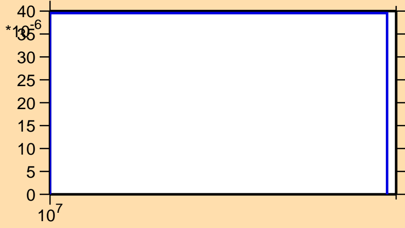
\sigma vs. E for ^{125}\text{Pr}(n,2n)
