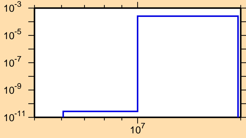
\sigma vs. E for ^{125}\text{Pr}(n,t)
