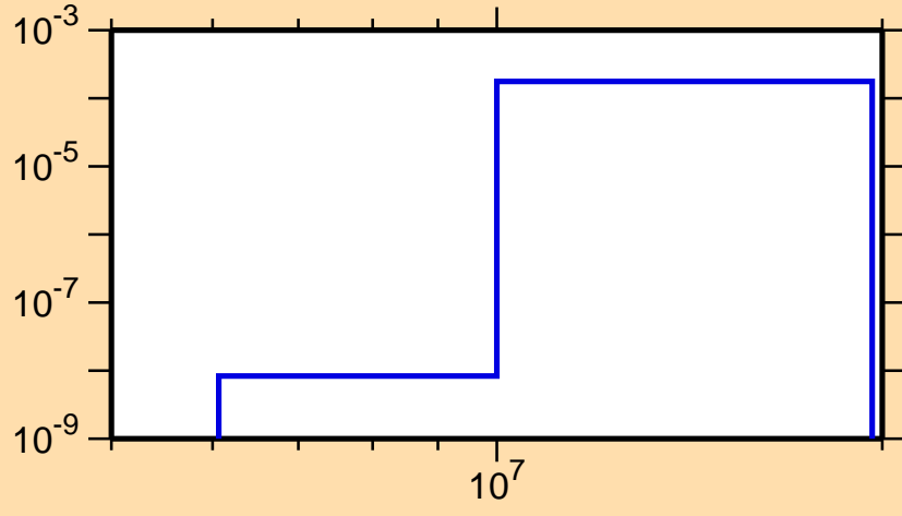
\sigma vs. E for ^{125}\text{Pr}(\text{mt } 45)
