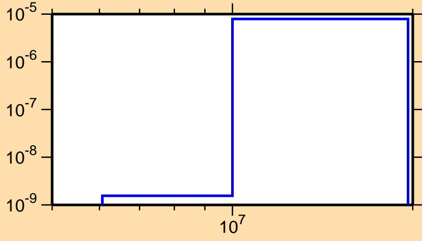
\sigma vs. E for ^{125}\text{Pr}(\text{mt117})
