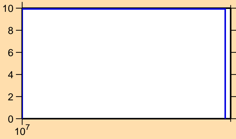
\Delta\sigma/\sigma vs. E for ^{125}\text{Pr}(n,\text{inel.})
