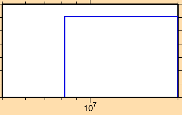
\sigma vs. E for ^{125}\text{Pr}(n,\text{nd})
