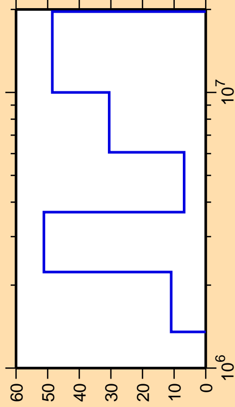
\Delta\sigma/\sigma vs. E for ^{126}\text{Pr}(n,np)
