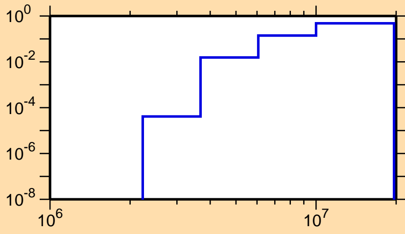
\sigma vs. E for ^{126}\text{Pr}(n,np)
