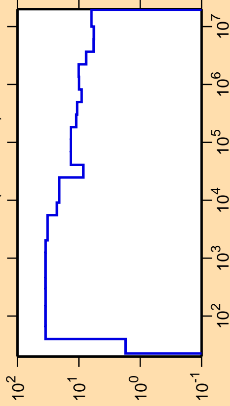
\Delta\sigma/\sigma vs. E for ^{126}\text{Pr}(n,\text{nonel.})
