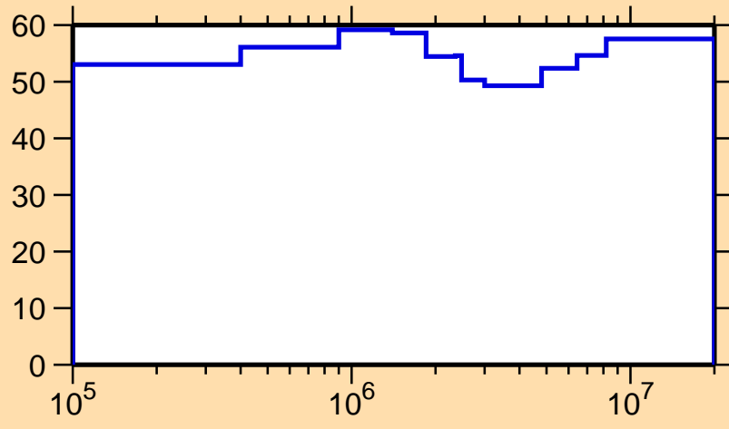
\Delta\sigma/\sigma vs. E for ^{126}\text{Pr}(n,n_1)
