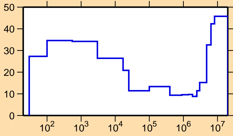
\Delta\sigma/\sigma vs. E for ^{126}\text{Pr}(n,p)
