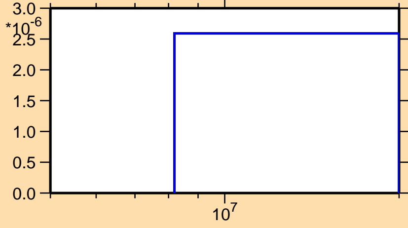
\sigma vs. E for ^{126}\text{Pr}(n,\text{nd})
