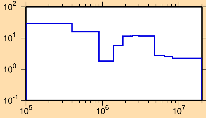
\Delta\sigma/\sigma vs. E for ^{126}\text{Pr}(n, el.)
