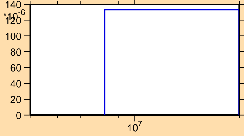
\sigma vs. E for ^{126}\text{Pr}(n,2np)
