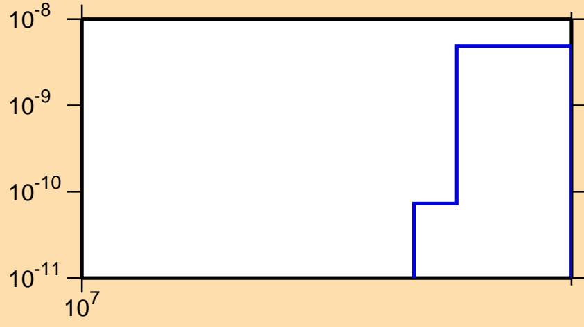
\sigma vs. E for ^{127}\text{Pr}(n,2n\alpha)
