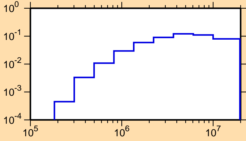
\sigma vs. E for ^{127}\text{Pr}(n,n\text{cont.})
