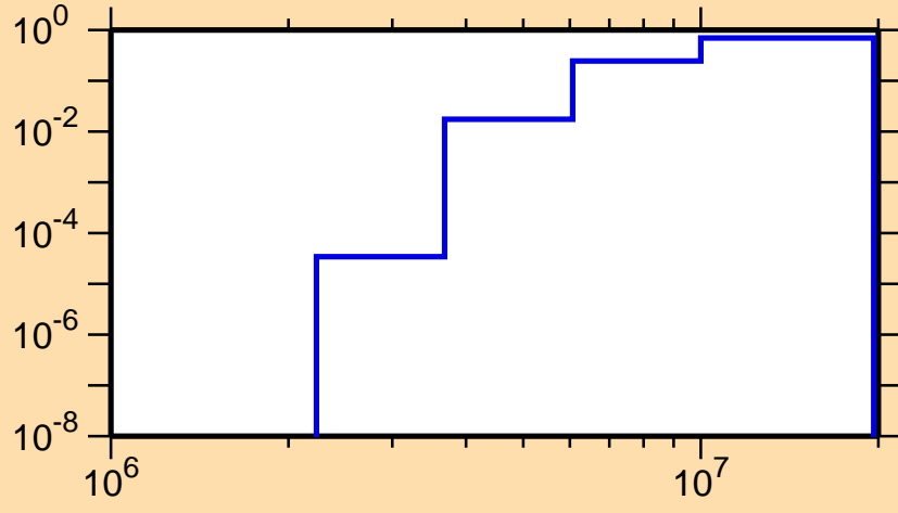
\sigma vs. E for ^{127}\text{Pr}(n,np)
