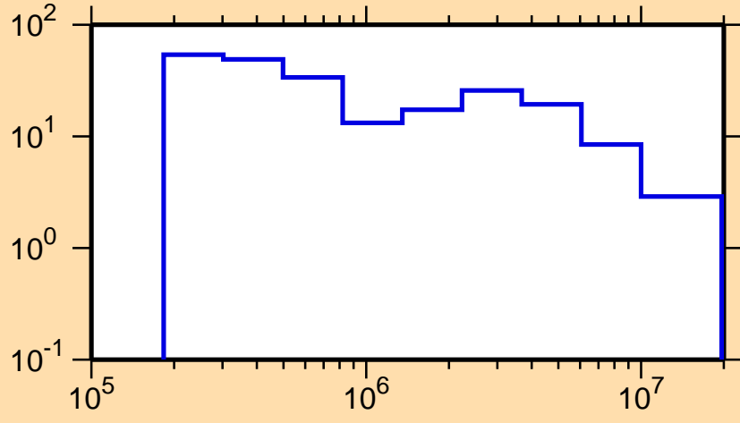
\Delta\sigma/\sigma vs. E for ^{127}\text{Pr}(n, el.)
