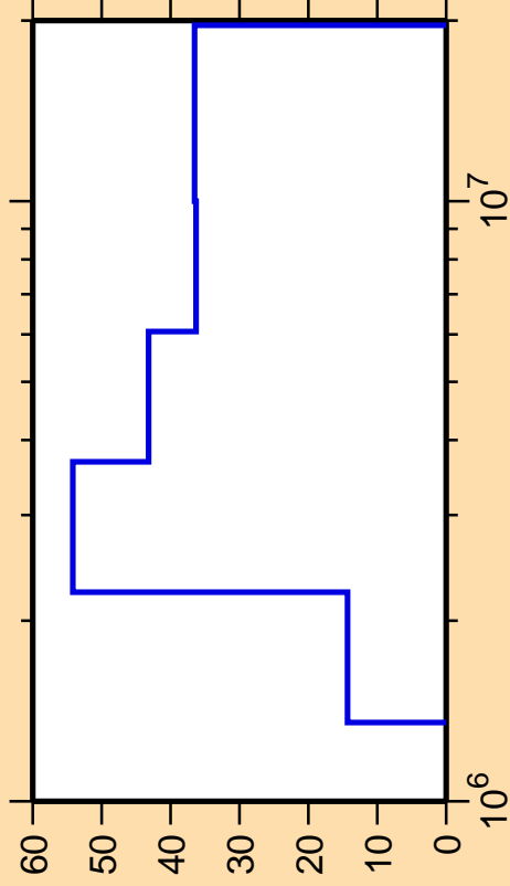
\Delta\sigma/\sigma vs. E for ^{127}\text{Pr}(n,np)
