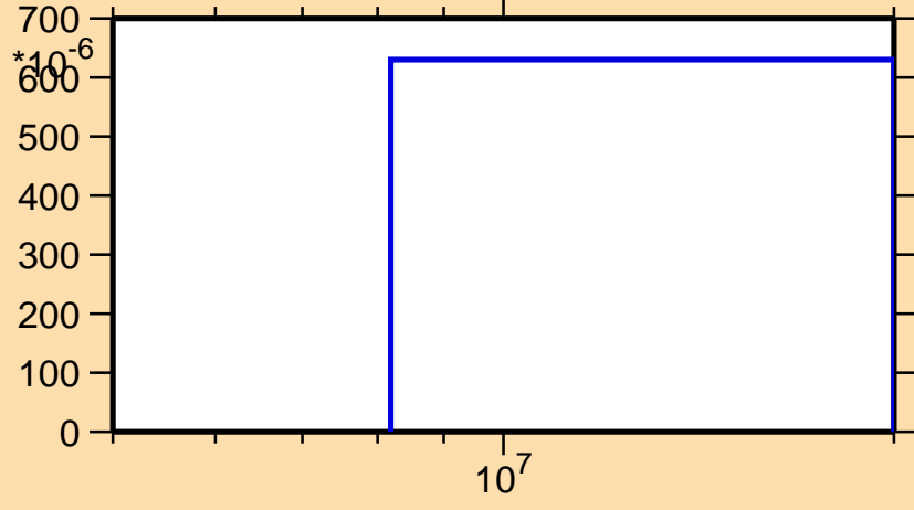
\sigma vs. E for ^{127}\text{Pr}(n,2n)
