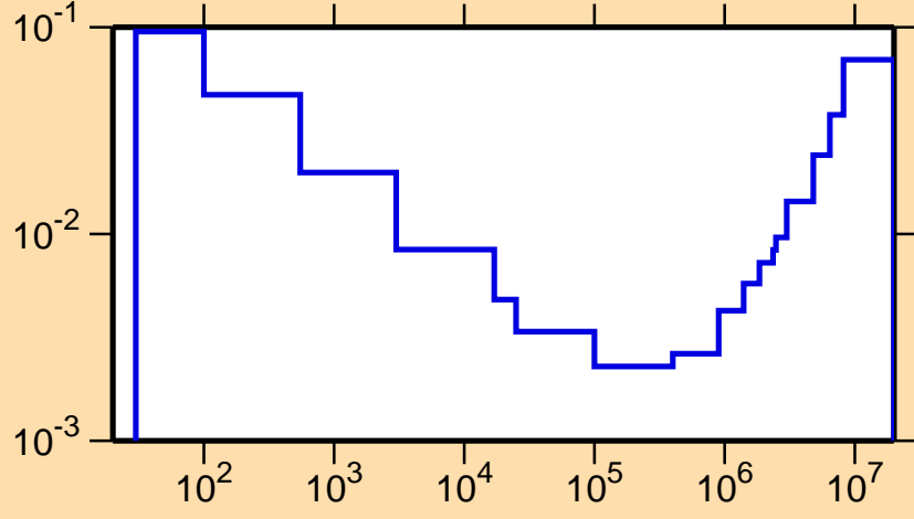
\sigma vs. E for ^{127}\text{Pr}(n,\alpha)
