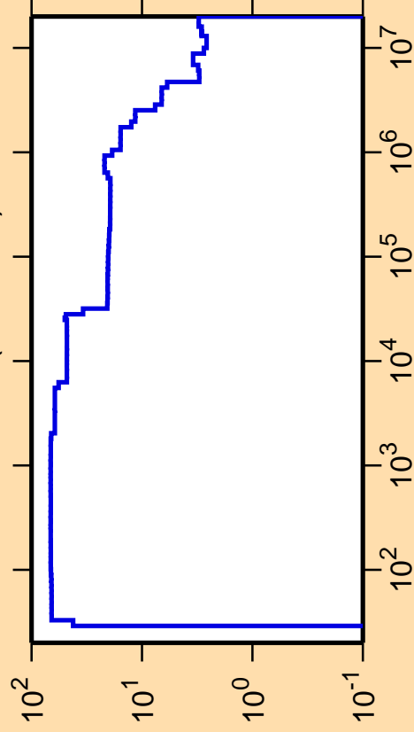
\Delta\sigma/\sigma vs. E for ^{128}\text{Pr}(n,\text{nonel.})
