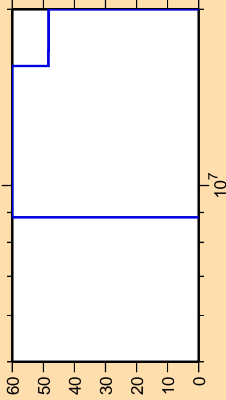
\Delta\sigma/\sigma vs. E for ^{128}\text{Pr}(n,2n)
