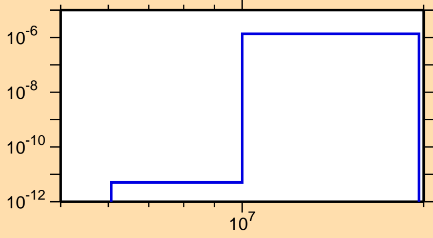
\sigma vs. E for ^{128}\text{Pr}(\text{mt117})
