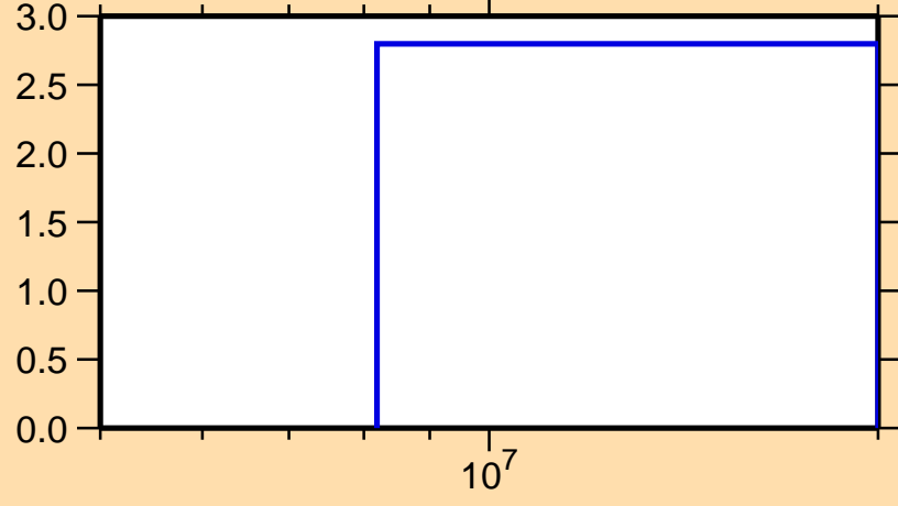
\Delta\sigma/\sigma vs. E for ^{128}\text{Pr}(n,\text{nonel.})
