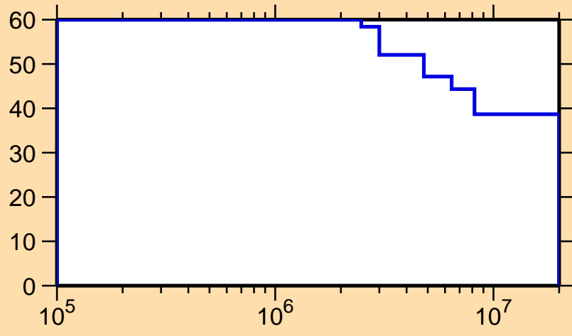
\Delta\sigma/\sigma vs. E for ^{128}\text{Pr}(n,n\text{cont.})
