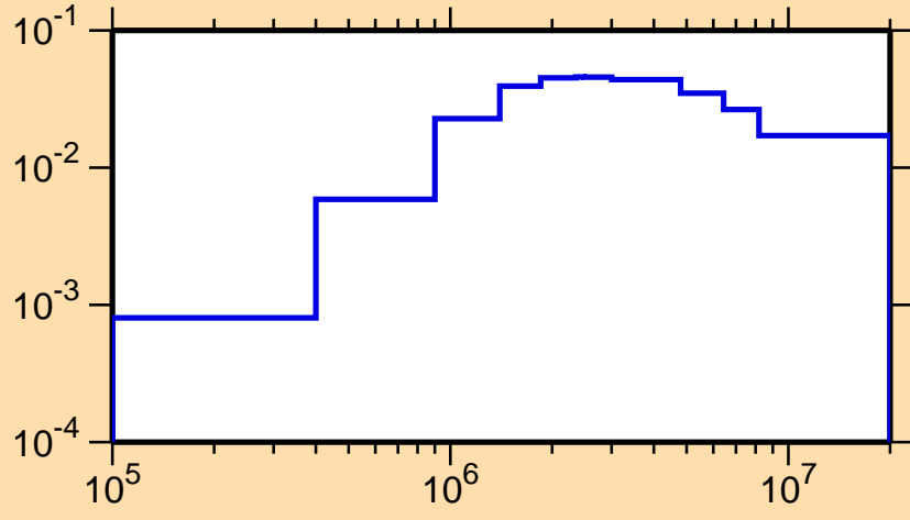
\sigma vs. E for ^{128}\text{Pr}(n,n_1)
