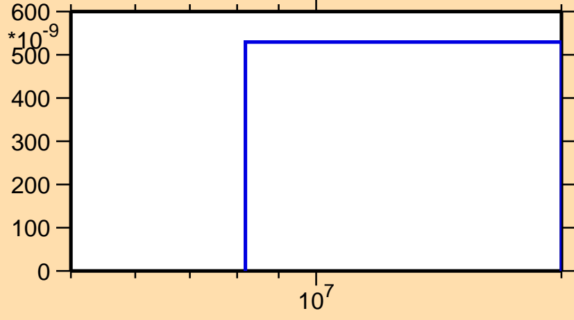
\sigma vs. E for ^{128}\text{Pr}(n,\text{pt})
