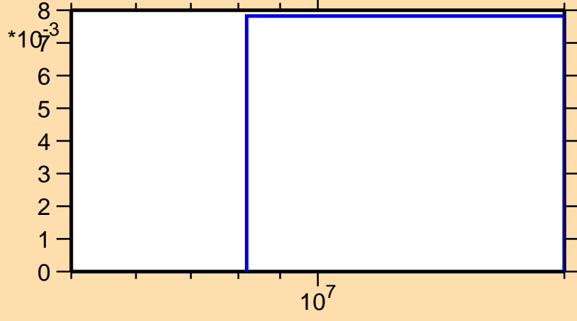
\sigma vs. E for ^{128}\text{Pr}(n,2n)
