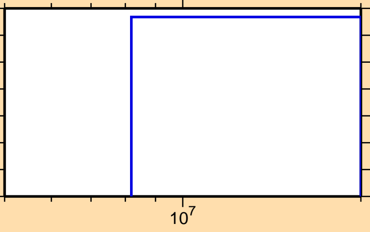
\sigma vs. E for ^{128}\text{Pr}(\text{mt } 34)
