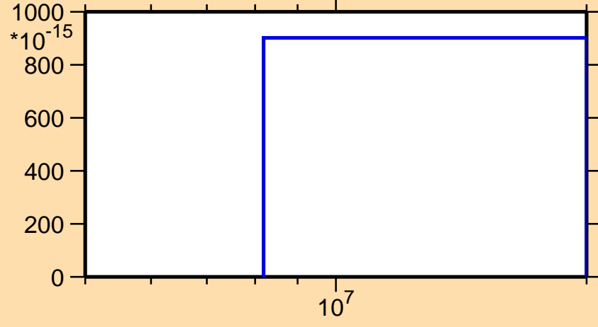
\sigma vs. E for ^{128}\text{Pr}(n,nt)
