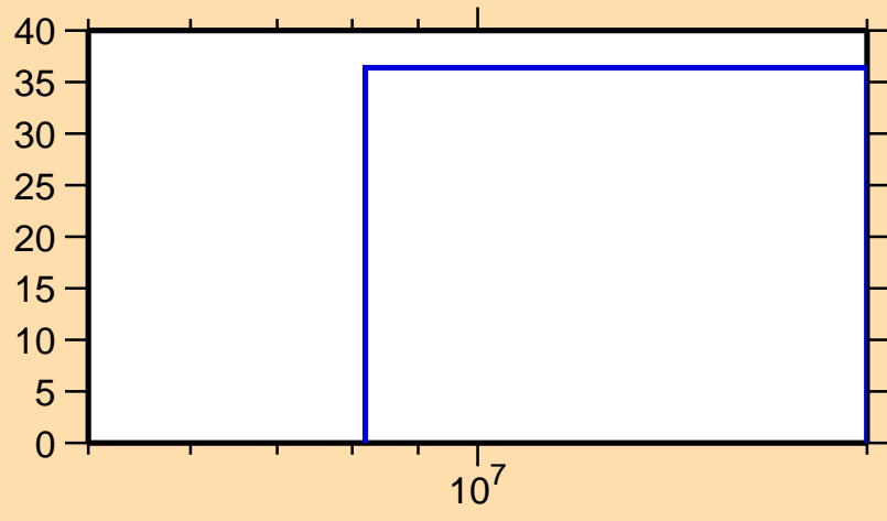
\Delta\sigma/\sigma vs. E for ^{128}\text{Pr}(n,\text{inel.})
