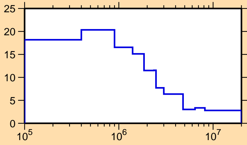
\Delta\sigma/\sigma vs. E for ^{128}\text{Pr}(n,\text{nonel.})
