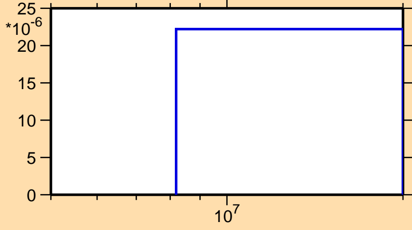
\sigma vs. E for ^{128}\text{Pr}(n,\text{pd})
