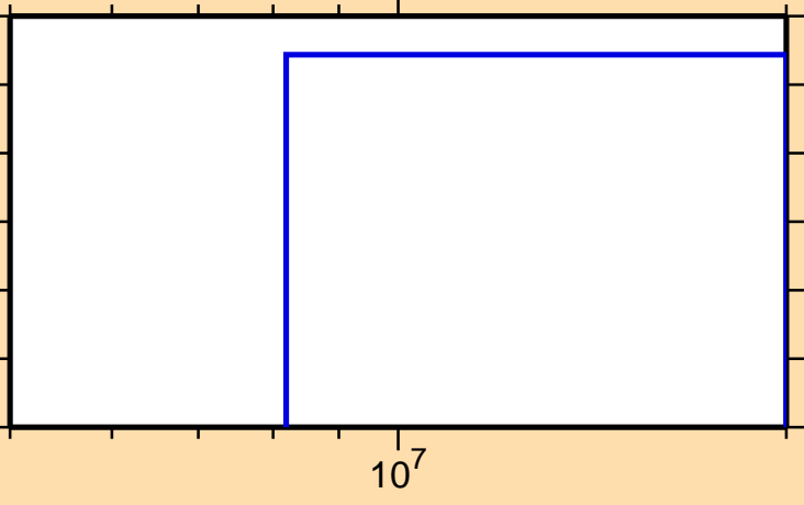
\sigma vs. E for ^{128}\text{Pr}(n,2np)
