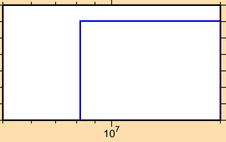
\sigma vs. E for ^{128}\text{Pr}(n,\text{nd})
