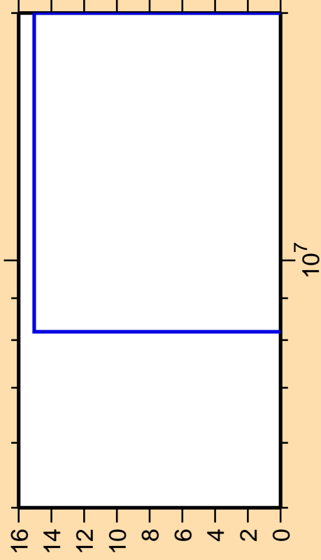
\Delta\sigma/\sigma vs. E for ^{128}\text{Pr}(n,n_1)
