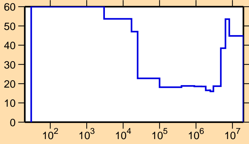
\Delta\sigma/\sigma vs. E for ^{128}\text{Pr}(n,p)
