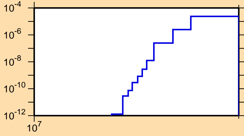
\sigma vs. E for ^{129}\text{Pr}(n,nd)
