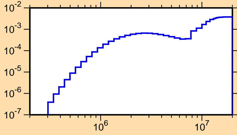
\sigma vs. E for ^{129}\text{Pr}(n,\text{inel.})
