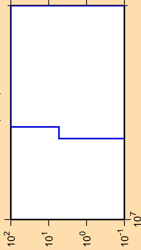
\Delta\sigma/\sigma vs. E for ^{129}\text{Pr}(n,nd)
