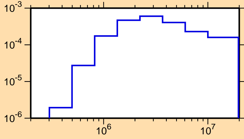
\sigma vs. E for ^{129}\text{Pr}(n,n_1)
