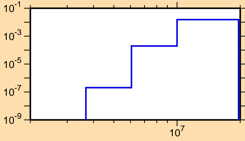
\sigma vs. E for ^{129}\text{Pr}(n,n\alpha)
