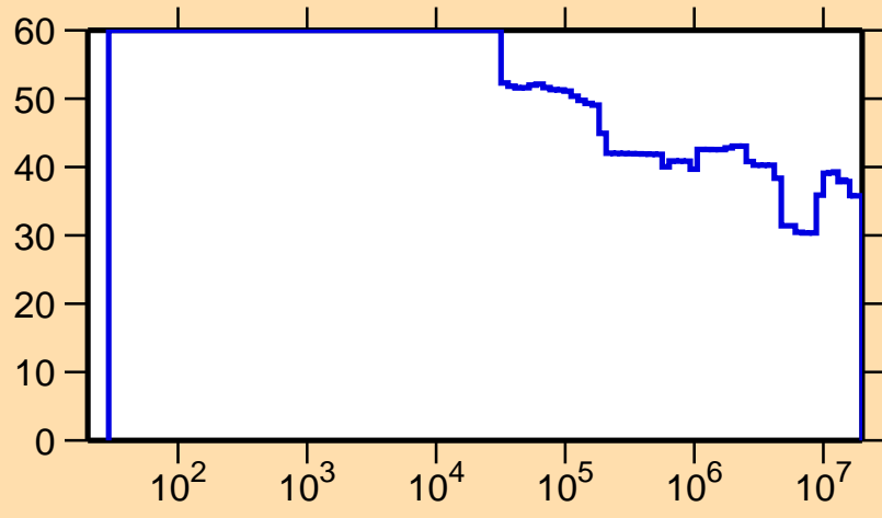
\Delta\sigma/\sigma vs. E for ^{130}\text{Pr}(n,p)
