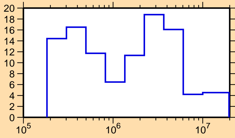
\Delta\sigma/\sigma vs. E for ^{130}\text{Pr}(n, el.)
