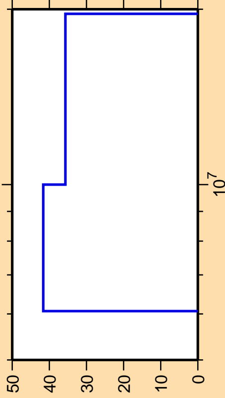
\Delta\sigma/\sigma vs. E for ^{130}\text{Pr}(n,n_1)
