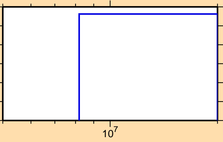
\sigma vs. E for ^{130}\text{Pr}(n,\text{nd})
