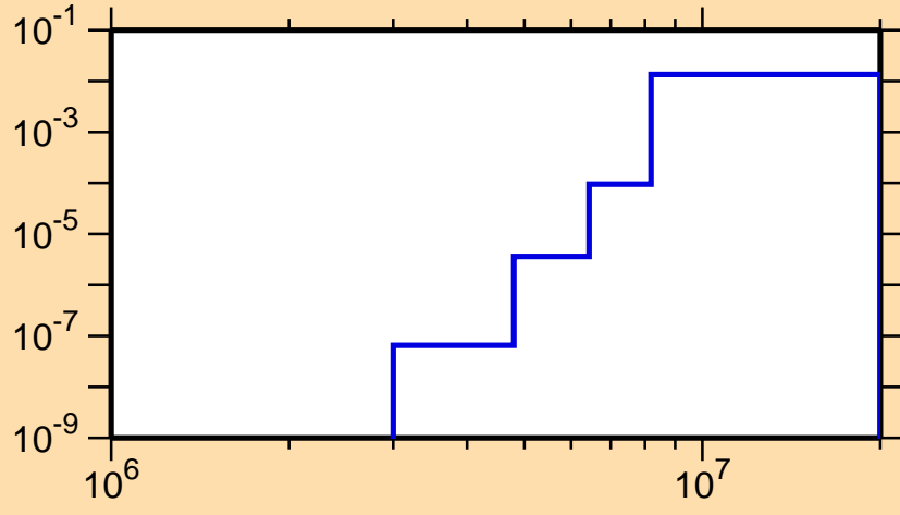
\sigma vs. E for ^{130}\text{Pr}(n,d)
