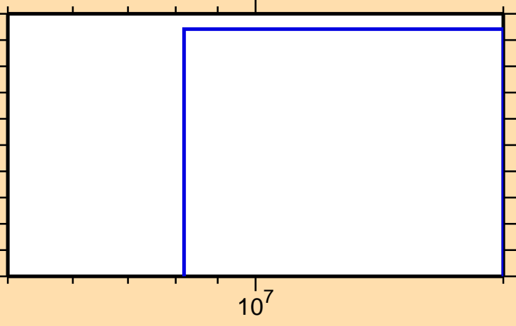
\sigma vs. E for ^{130}\text{Pr}(\text{mt } 45)
