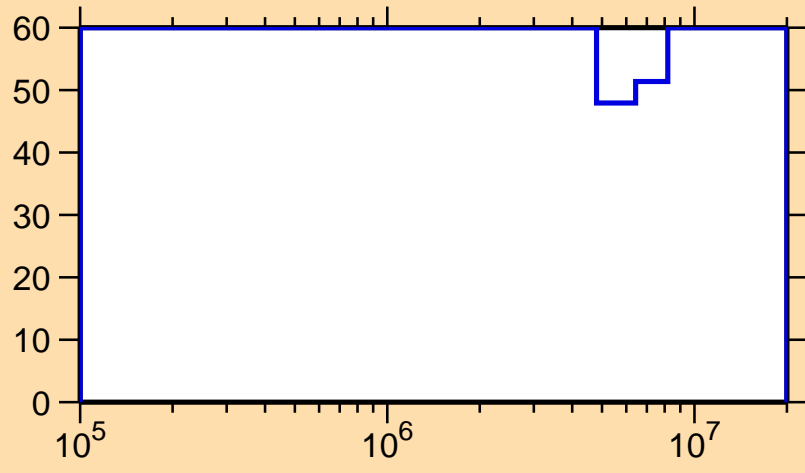
\Delta\sigma/\sigma vs. E for ^{130}\text{Pr}(n,n\text{cont.})
