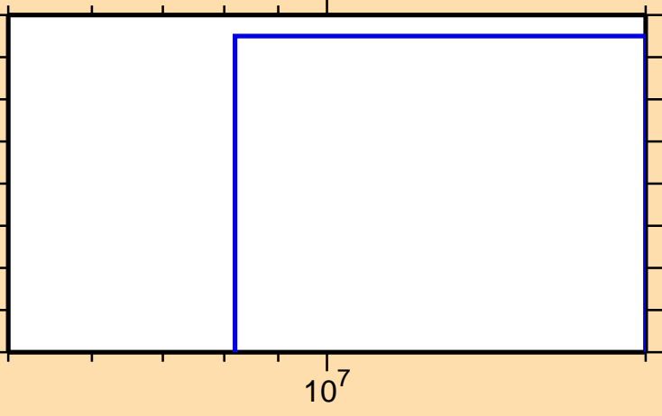
\sigma vs. E for ^{131}\text{Pr}(n,\text{pt})
