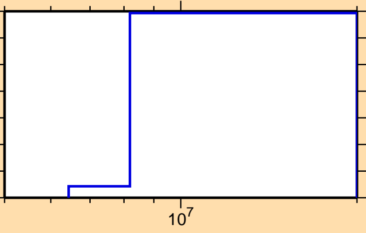
\sigma vs. E for ^{131}\text{Pr}(n,\text{He3})
