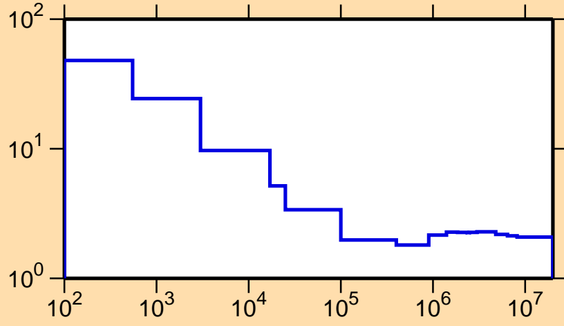
\sigma vs. E for ^{131}\text{Pr}(n,\text{nonel.})
