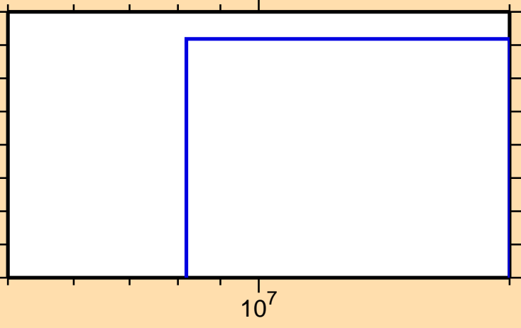
\sigma vs. E for ^{131}\text{Pr}(\text{mt117})
