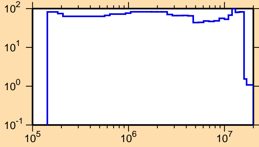
\Delta\sigma/\sigma vs. E for ^{132}\text{Pr}(n,n_1)
