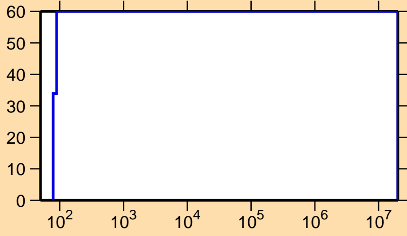
\Delta\sigma/\sigma vs. E for ^{132}\text{Pr}(n,p)
