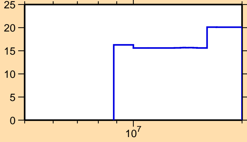
\Delta\sigma/\sigma vs. E for ^{132}\text{Pr}(n,\text{nonel.})
