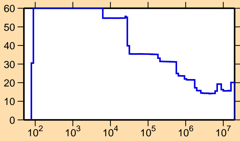
\Delta\sigma/\sigma vs. E for ^{132}\text{Pr}(n,\text{nonel.})
