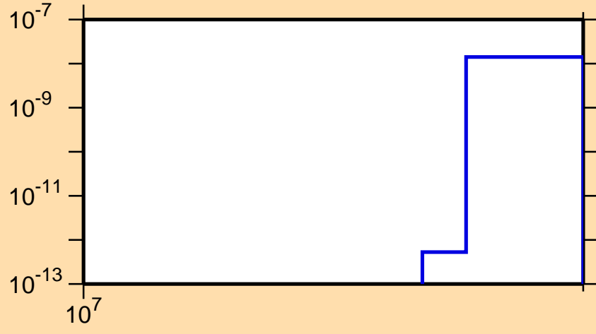
\sigma vs. E for ^{132}\text{Pr}(n,nt)
