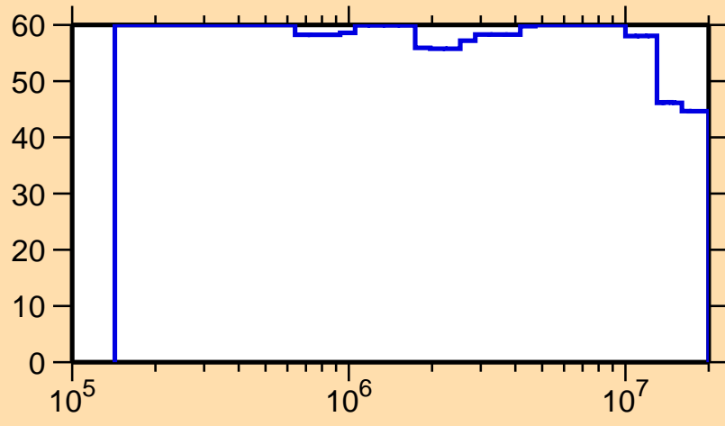
\Delta\sigma/\sigma vs. E for ^{132}\text{Pr}(n,\text{inel.})
