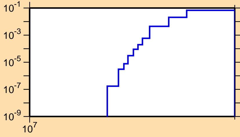
\sigma vs. E for ^{132}\text{Pr}(n,2np)
