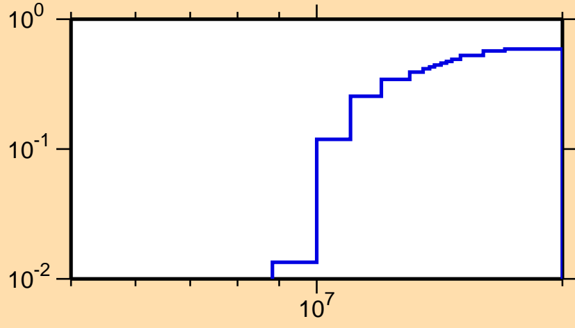
\sigma vs. E for ^{132}\text{Pr}(n,2n)
