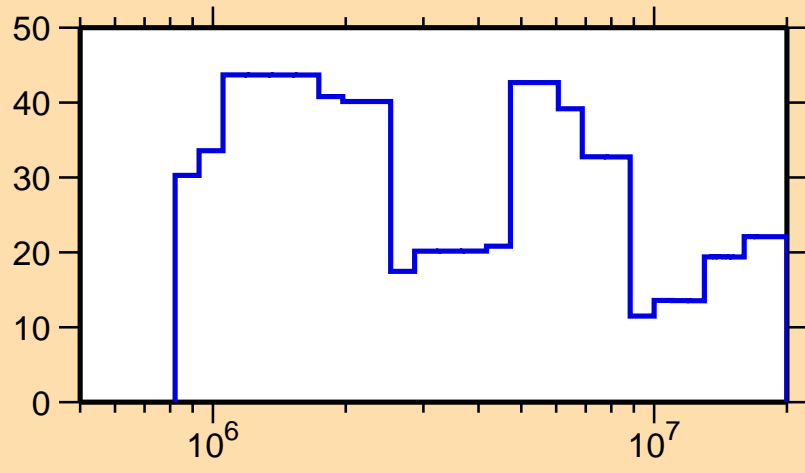
\Delta\sigma/\sigma vs. E for ^{132}\text{Pr}(n,\text{el.})
