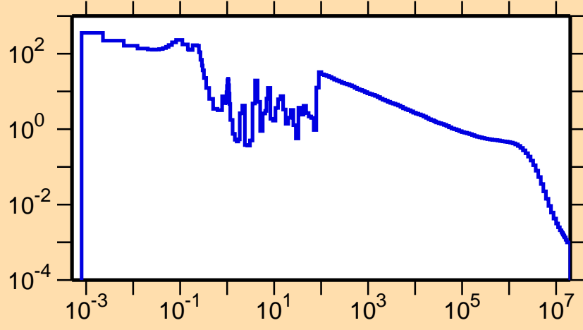
\sigma vs. E for ^{132}\text{Pr}(n,\gamma)
