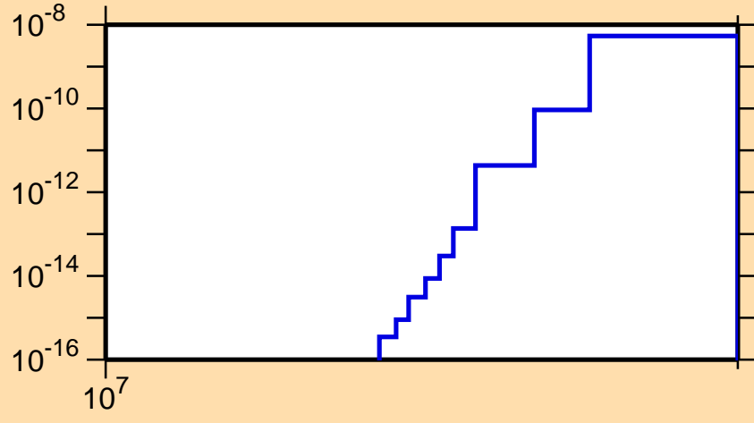
\sigma vs. E for ^{132}\text{Pr}(\text{mt } 34)
