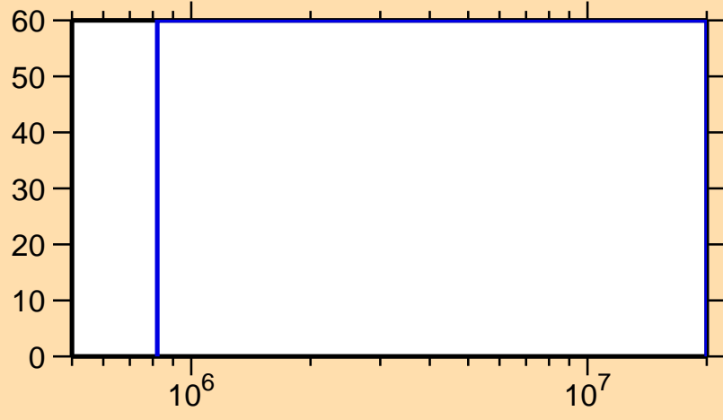
\Delta\sigma/\sigma vs. E for ^{132}\text{Pr}(n,n\text{cont.})
