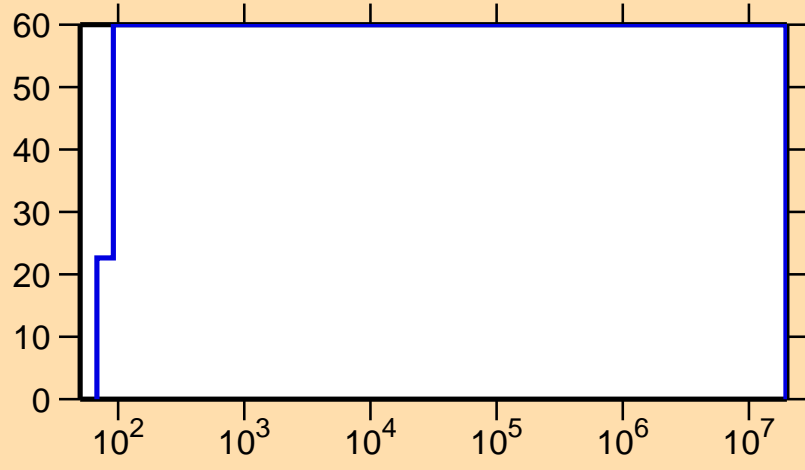
\Delta\sigma/\sigma vs. E for ^{132}\text{Pr}(n,p)
