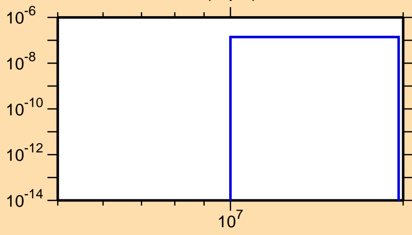
\sigma vs. E for ^{132}\text{Pr}(n,pd)
