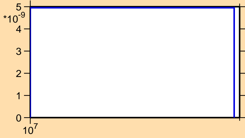
\sigma vs. E for ^{132}\text{Pr}(n,\text{pt})
