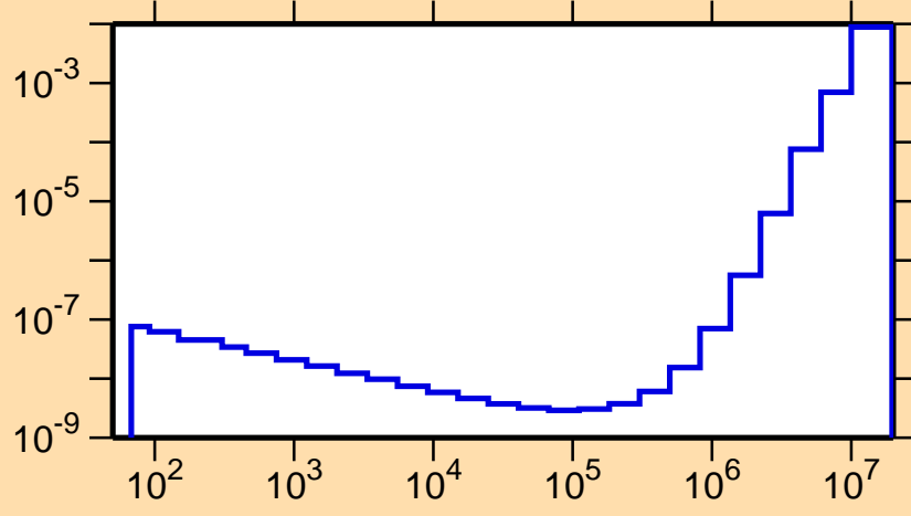
\sigma vs. E for ^{132}\text{Pr}(n,p\alpha)
