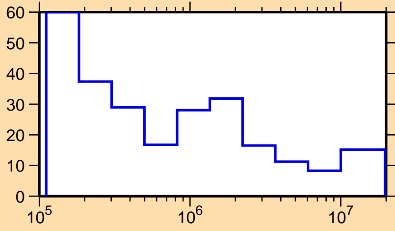
\Delta\sigma/\sigma vs. E for ^{132}\text{Pr}(n,\text{tot.})
