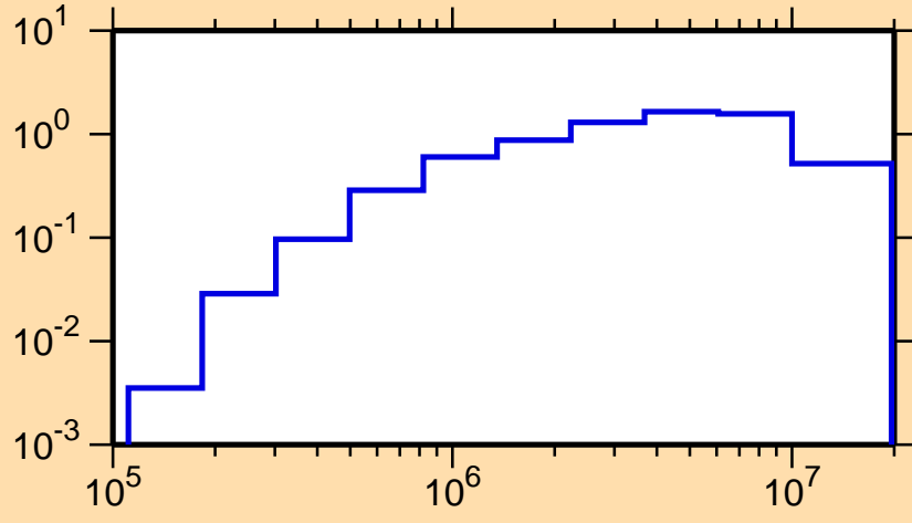
\sigma vs. E for ^{132}\text{Pr}(n,\text{inel.})
