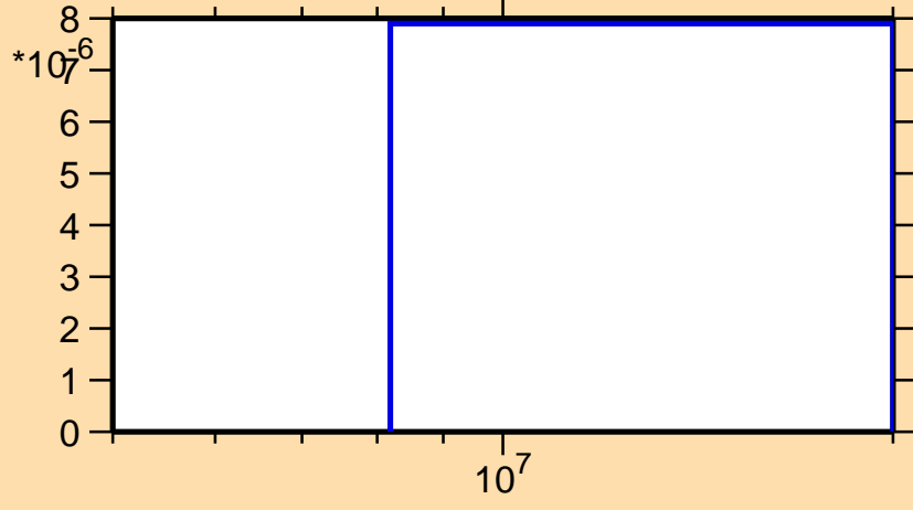
\sigma vs. E for ^{132}\text{Pr}(n,\text{nd})
