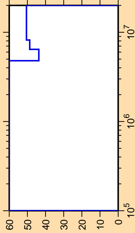
\Delta\sigma/\sigma vs. E for ^{132}\text{Pr}(n,n_1)
