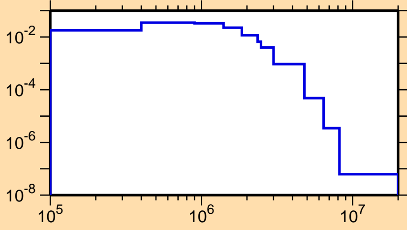
\sigma vs. E for ^{132}\text{Pr}(n,n_1)
