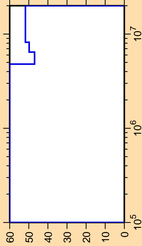
\Delta\sigma/\sigma vs. E for ^{132}\text{Pr}(n,n_2)
