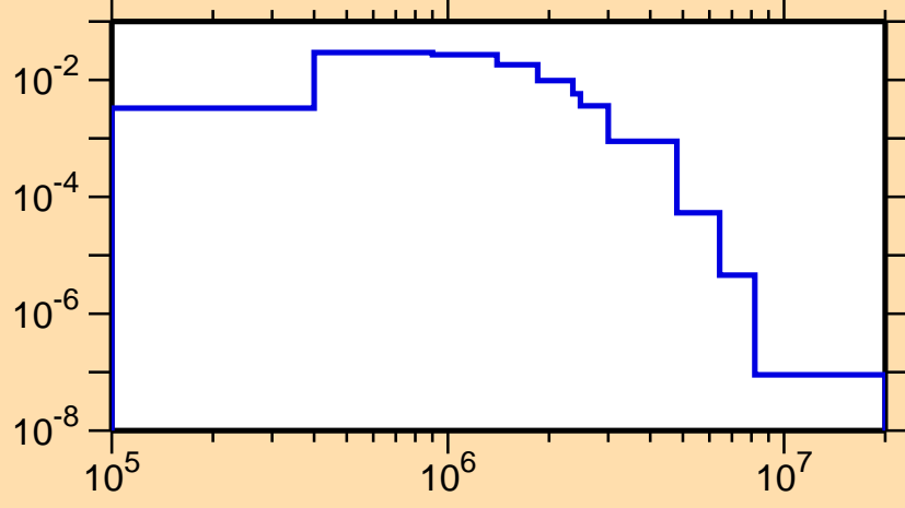
\sigma vs. E for ^{132}\text{Pr}(n,n_2)
