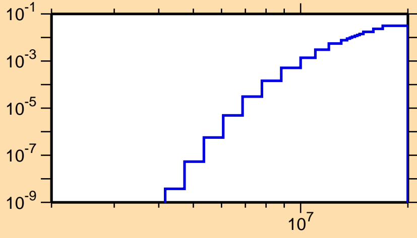
\sigma vs. E for ^{133}\text{Pr}(n,n\alpha)
