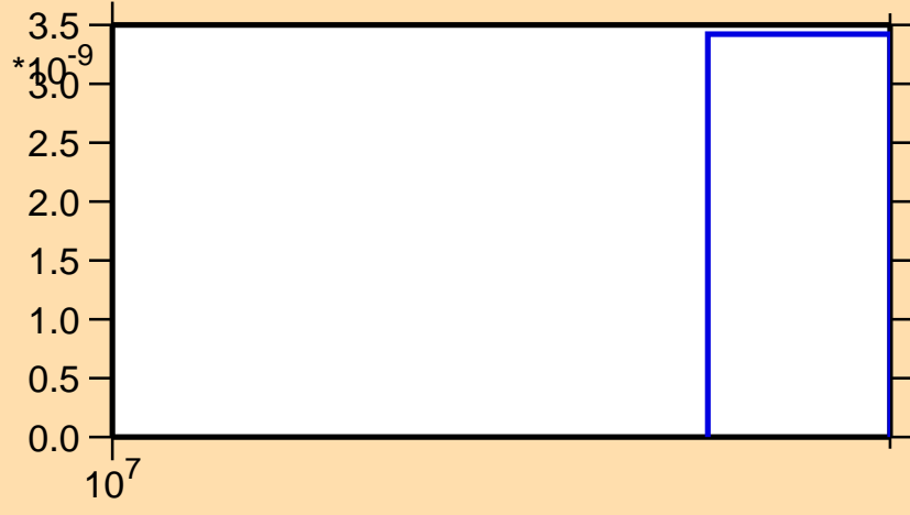
\sigma vs. E for ^{133}\text{Pr}(n,3n)
