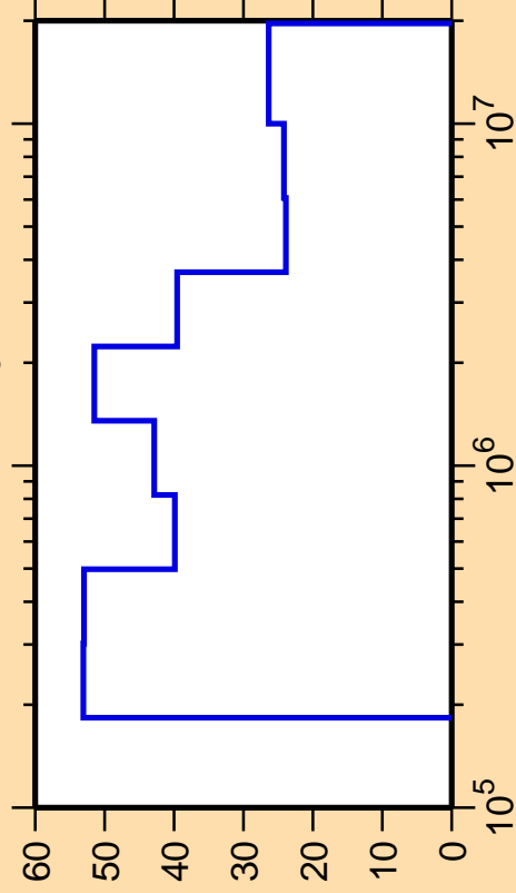
\Delta\sigma/\sigma vs. E for ^{133}\text{Pr}(n,n_3)
