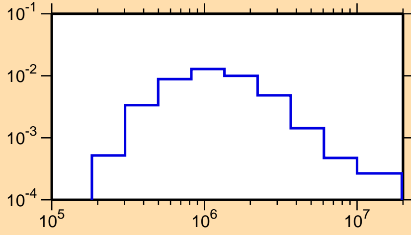
\sigma vs. E for ^{133}\text{Pr}(n,n_3)
