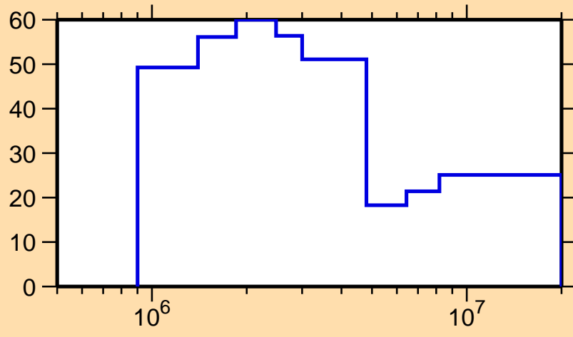
\Delta\sigma/\sigma vs. E for ^{133}\text{Pr}(n,n_1)
