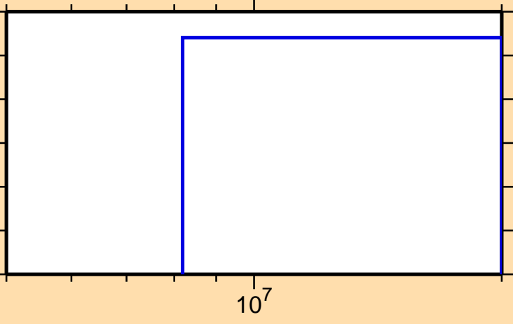
\sigma vs. E for ^{133}\text{Pr}(n,2n\alpha)
