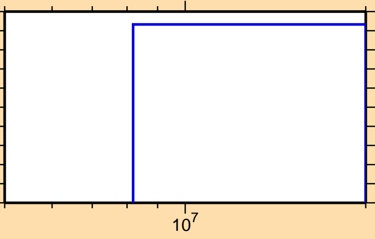
\sigma vs. E for ^{133}\text{Pr}(n,\text{He3})
