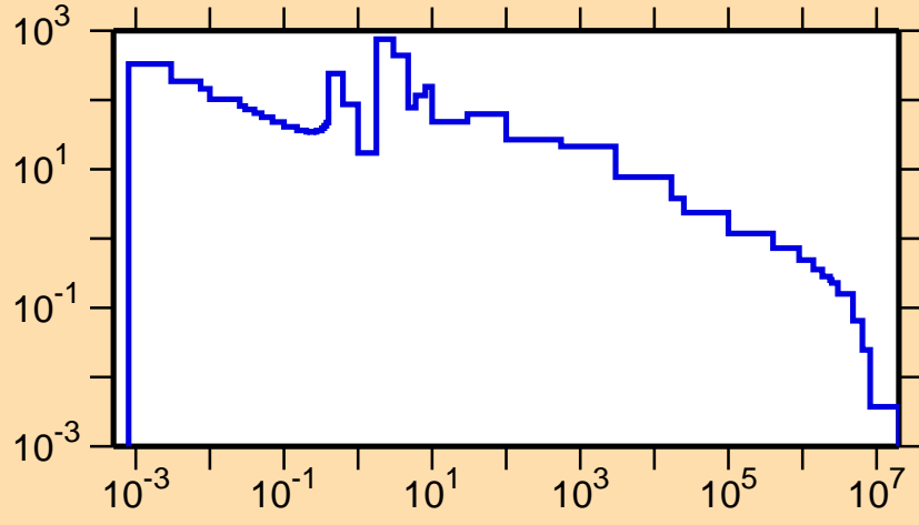
\sigma vs. E for ^{133}\text{Pr}(n,\gamma)
