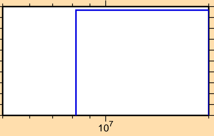
\sigma vs. E for ^{133}\text{Pr}(n,nt)
