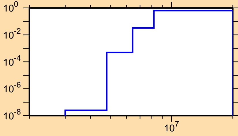
\sigma vs. E for ^{133}\text{Pr}(n,np)
