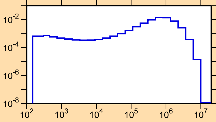
\sigma vs. E for ^{133}\text{Pr}(n,n_2)
