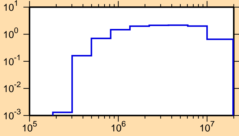
\sigma vs. E for ^{134}\text{Pr}(n,\text{inel.})
