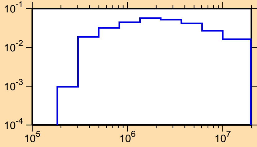
\sigma vs. E for ^{134}\text{Pr}(n,n_2)
