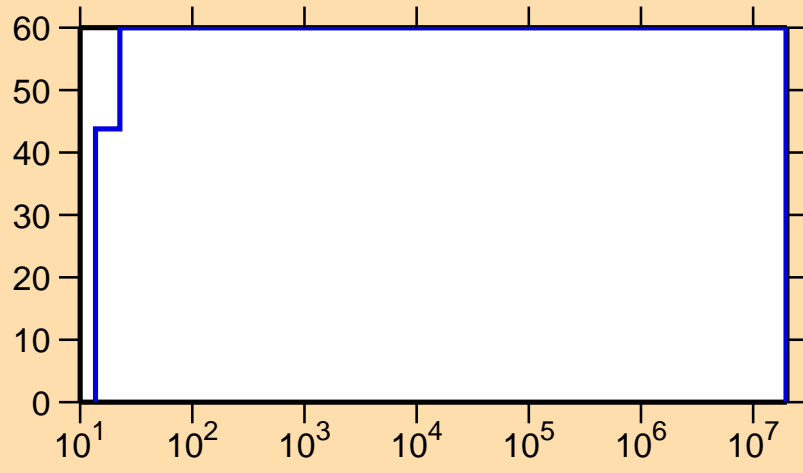
\Delta\sigma/\sigma vs. E for ^{134}\text{Pr}(n,\gamma)
