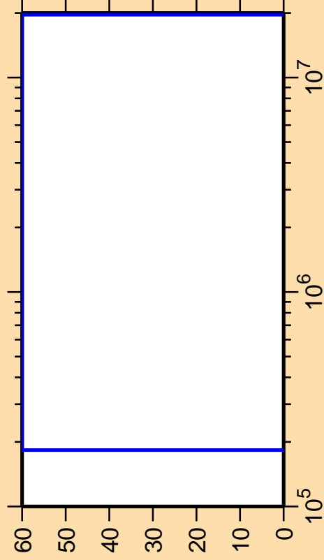
\Delta\sigma/\sigma vs. E for ^{134}\text{Pr}(n,\gamma)
