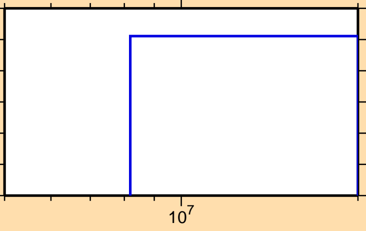
\sigma vs. E for ^{134}\text{Pr}(\text{mt117})
