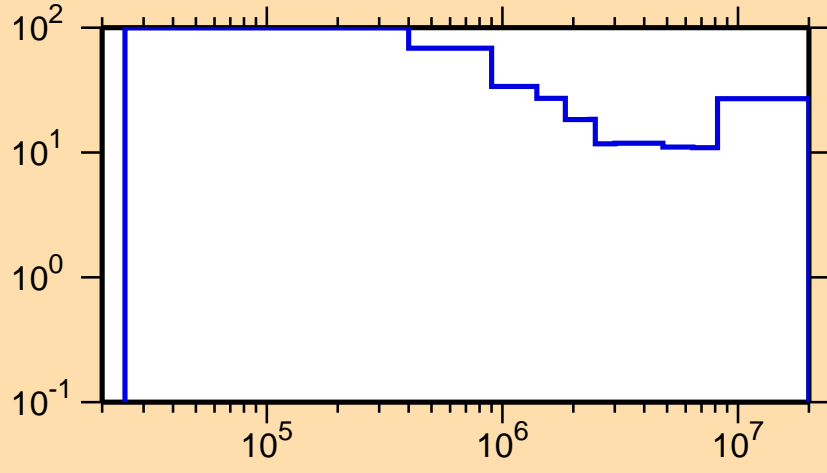
\Delta\sigma/\sigma vs. E for ^{135}\text{Pr}(n,\text{inel.})
