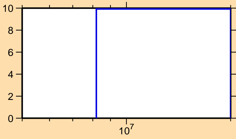
\Delta\sigma/\sigma vs. E for ^{135}\text{Pr}(n,\text{nonel.})
