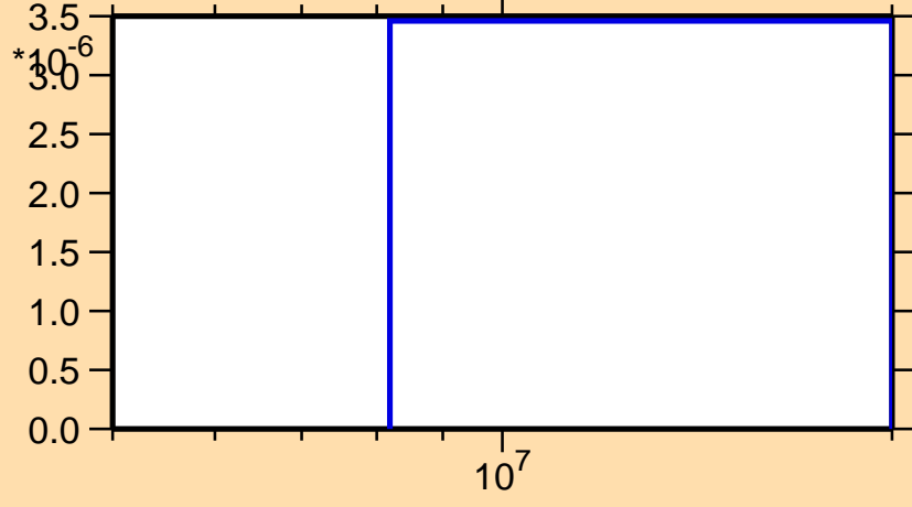
\sigma vs. E for ^{135}\text{Pr}(n,2np)
