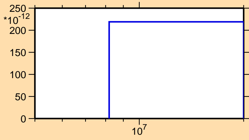
\sigma vs. E for ^{135}\text{Pr}(n,nt)
