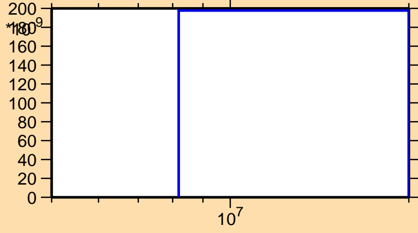
\sigma vs. E for ^{135}\text{Pr}(n,\text{He3})
