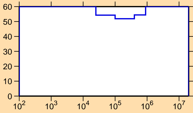
\Delta\sigma/\sigma vs. E for ^{135}\text{Pr}(n,\gamma)
