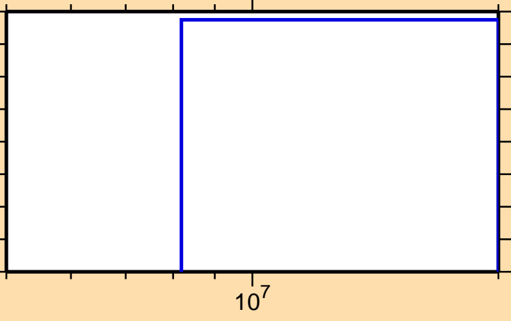
\sigma vs. E for ^{135}\text{Pr}(n,t)
