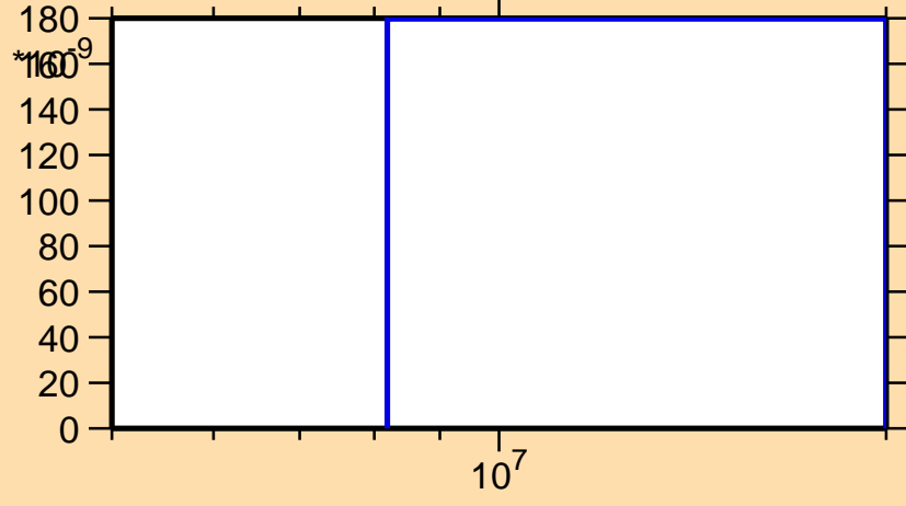
\sigma vs. E for ^{135}\text{Pr}(n,3n)
