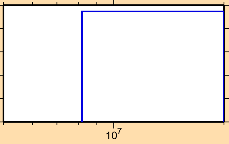
\sigma vs. E for ^{135}\text{Pr}(n,2n\alpha)
