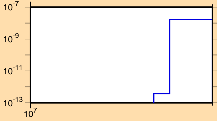
\sigma vs. E for ^{136}\text{Pr}(n,nt)
