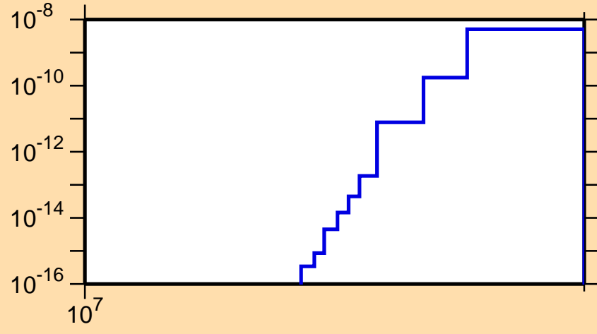
\sigma vs. E for ^{136}\text{Pr}(n,pd)
