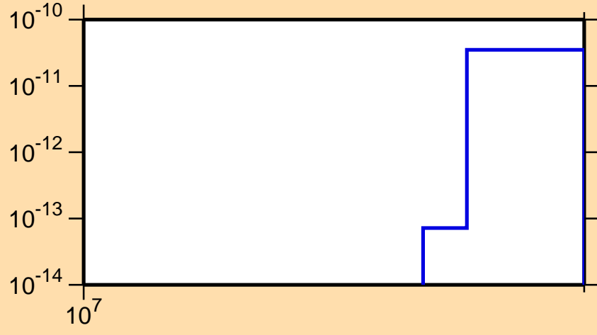
\sigma vs. E for ^{136}\text{Pr}(\text{mt } 34)
