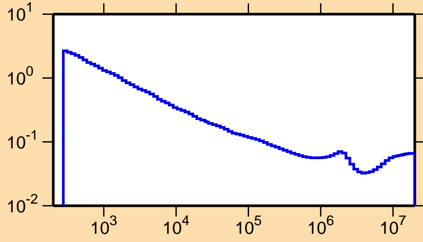
\sigma vs. E for ^{136}\text{Pr}(n,p)
