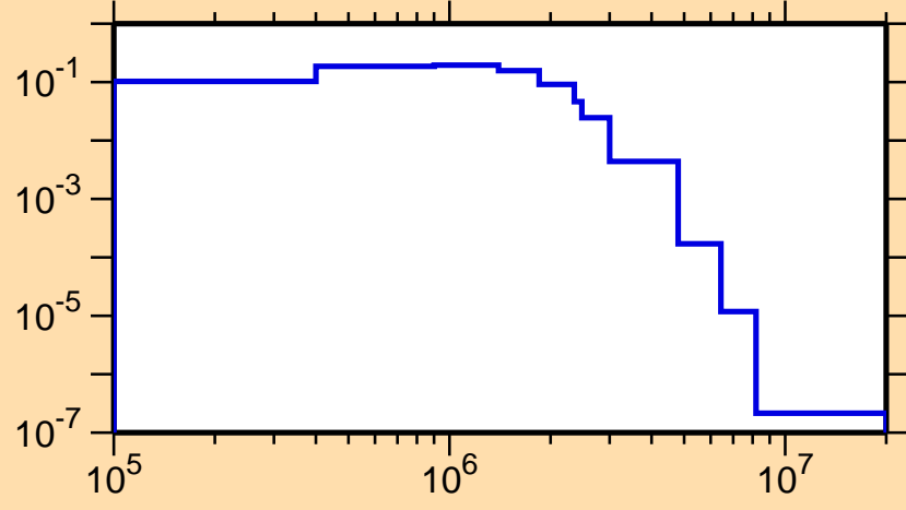
\sigma vs. E for ^{136}\text{Pr}(n,n_2)
