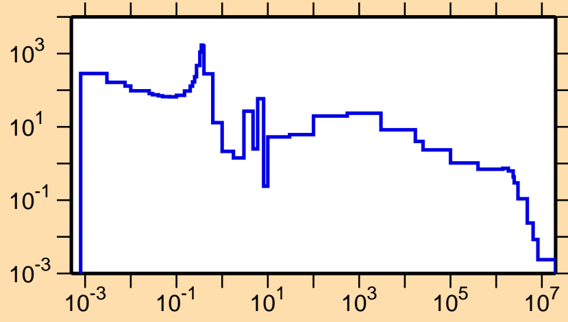
\sigma vs. E for ^{136}\text{Pr}(n,\gamma)
