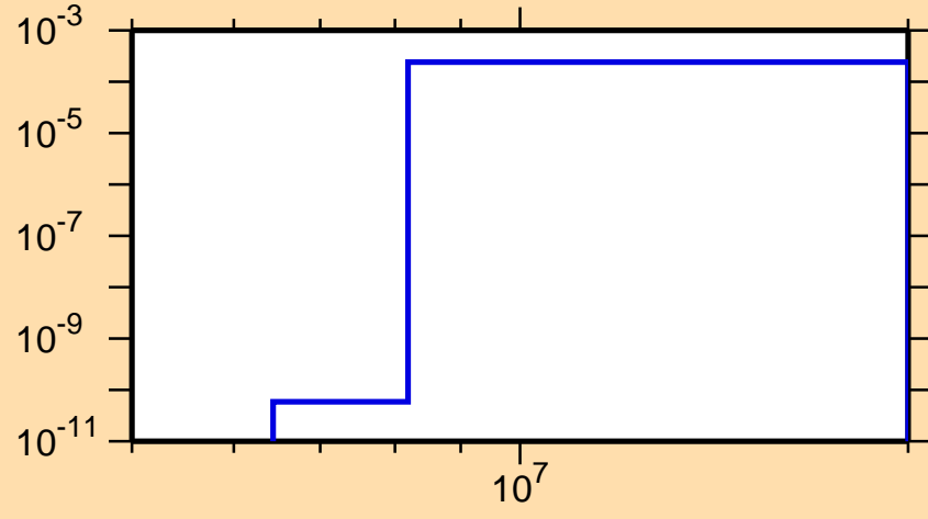
\sigma vs. E for ^{136}\text{Pr}(n,t)
