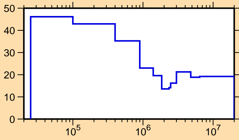
\Delta\sigma/\sigma vs. E for ^{136}\text{Pr}(n,n_1)
