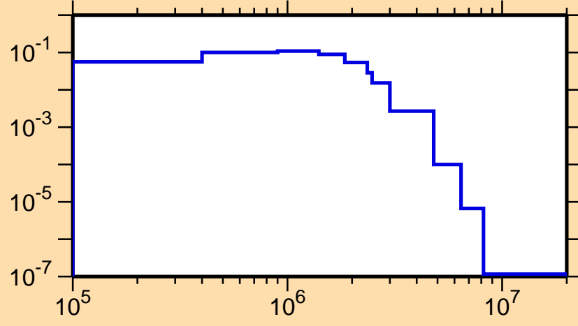
\sigma vs. E for ^{136}\text{Pr}(n,n_3)
