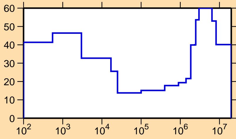
\Delta\sigma/\sigma vs. E for ^{136}\text{Pr}(n,\gamma)
