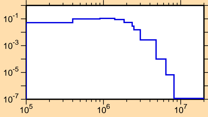
\sigma vs. E for ^{136}\text{Pr}(n,n_4)
