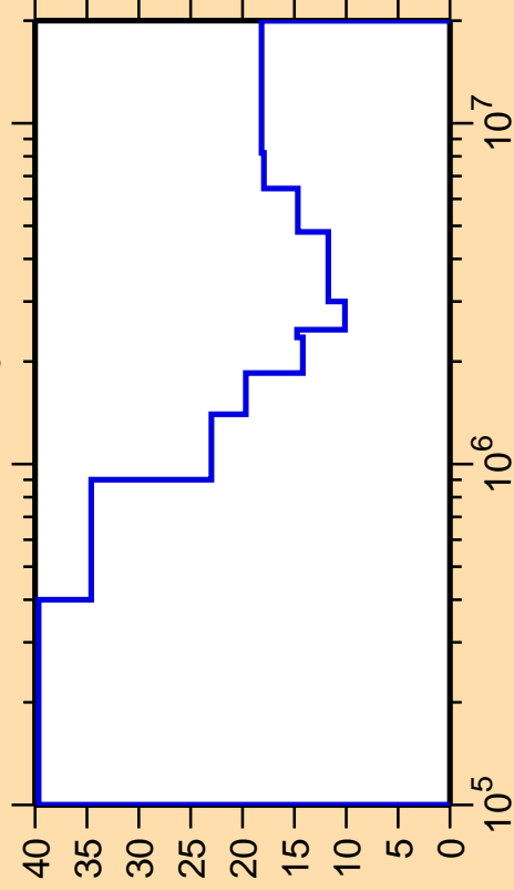
\Delta\sigma/\sigma vs. E for ^{136}\text{Pr}(n,n_3)
