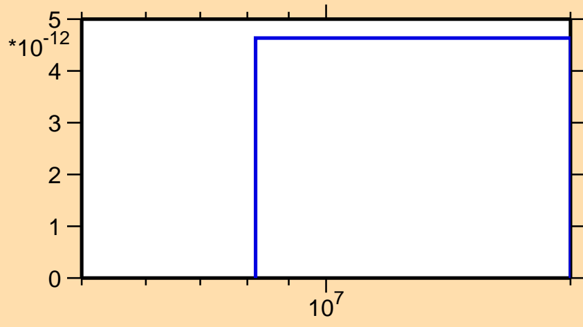
\sigma vs. E for ^{136}\text{Pr}(n,\text{pt})
