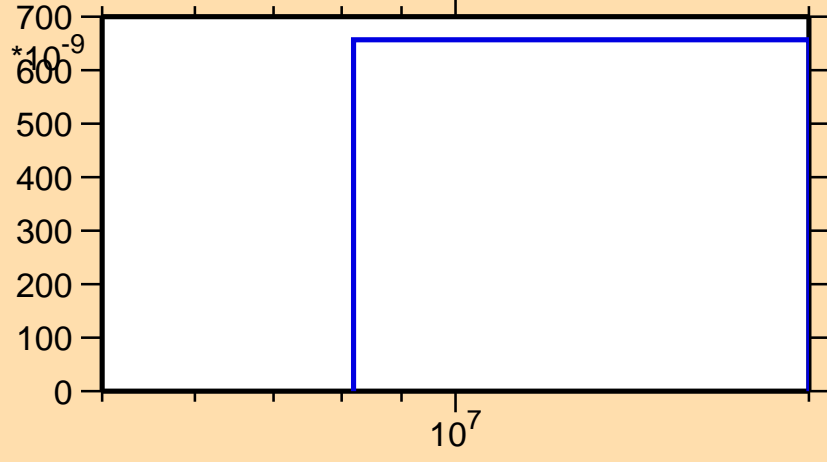
\sigma vs. E for ^{136}\text{Pr}(n,2n\alpha)
