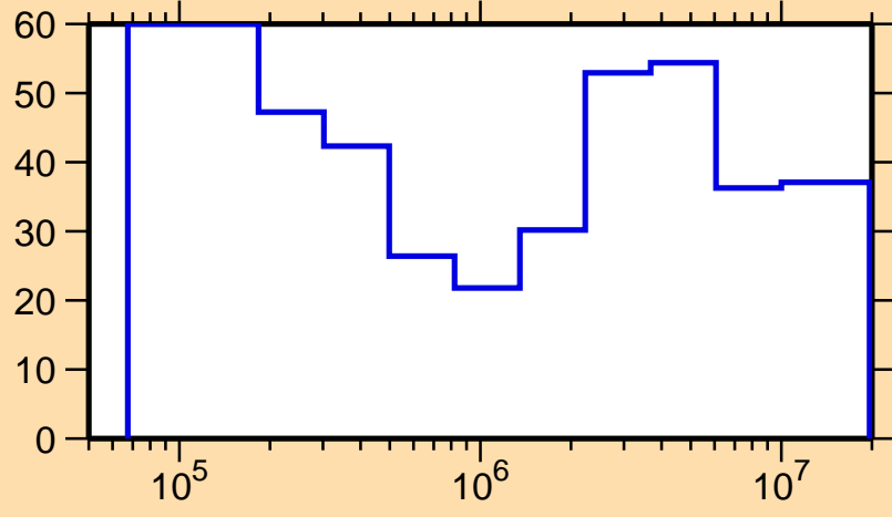
\Delta\sigma/\sigma vs. E for ^{137}\text{Pr}(n,n_1)
