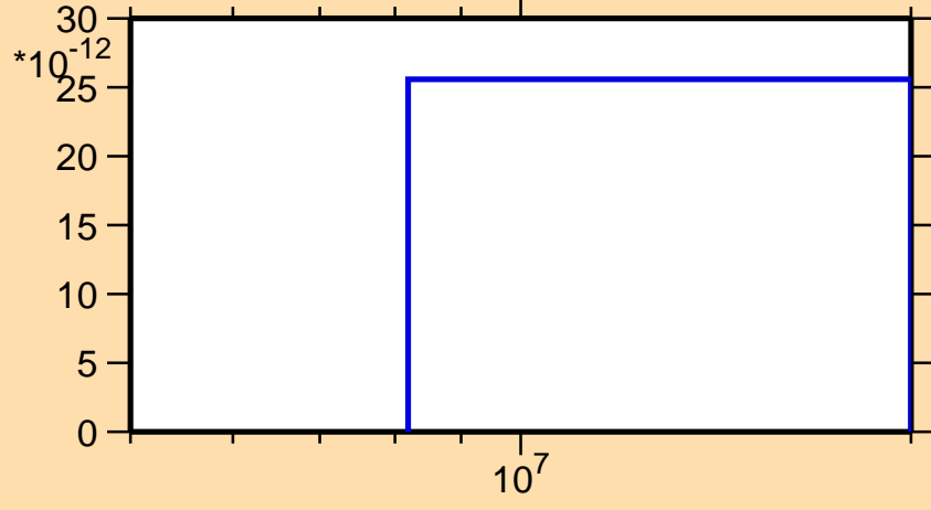
\sigma vs. E for ^{137}\text{Pr}(n,pd)
