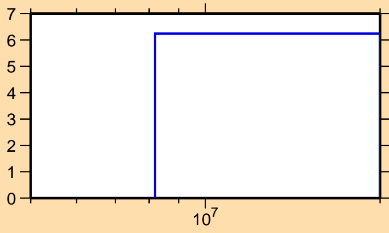
\Delta\sigma/\sigma vs. E for ^{137}\text{Pr}(n,\text{nonel.})
