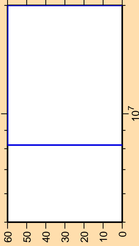
\Delta\sigma/\sigma vs. E for ^{137}\text{Pr}(\text{mt } 45)
