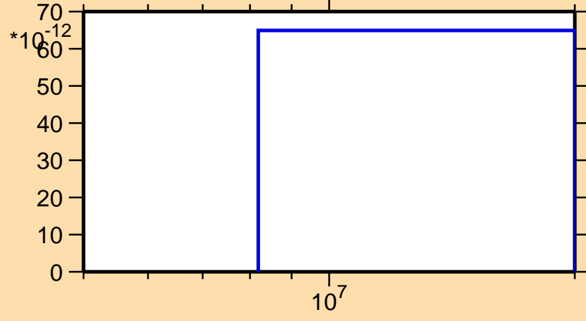
\sigma vs. E for ^{137}\text{Pr}(\text{mt117})
