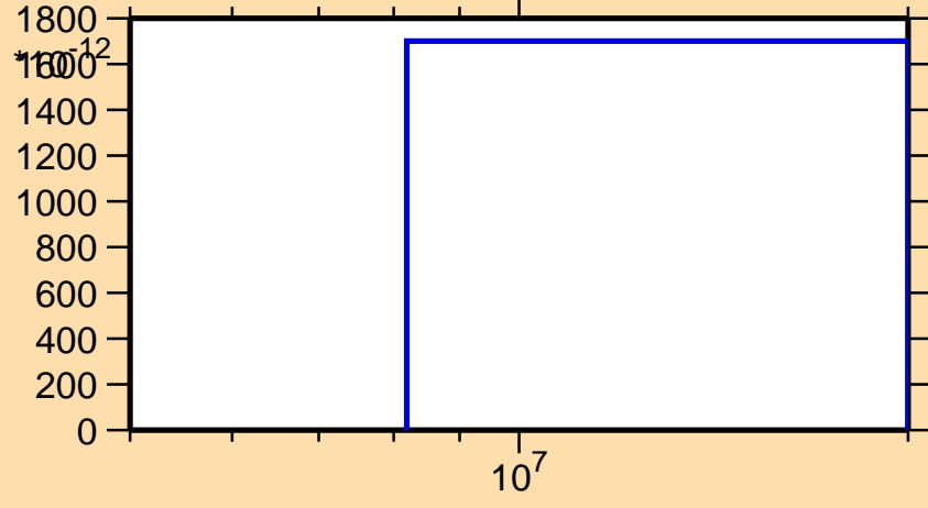
\sigma vs. E for ^{137}\text{Pr}(n,2n\alpha)
