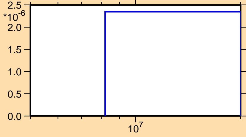
\sigma vs. E for ^{137}\text{Pr}(n,3n)
