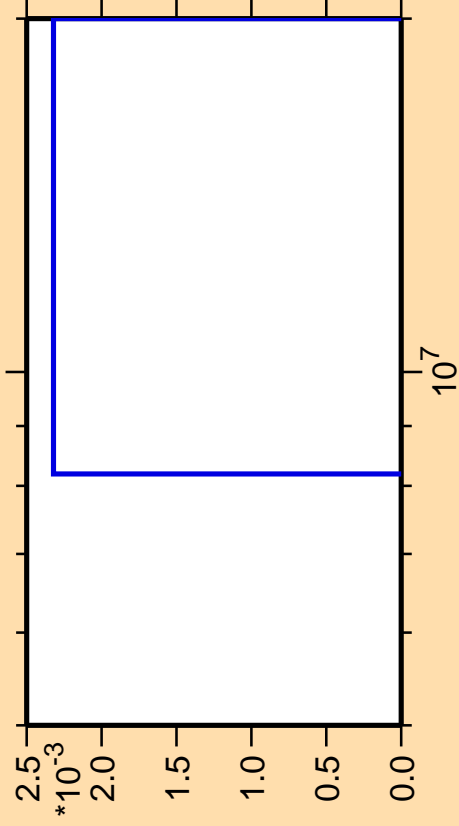
\Delta\sigma/\sigma vs. E for ^{137}\text{Pr}(n,\text{pt})
