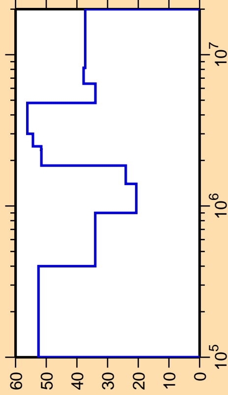
\Delta\sigma/\sigma vs. E for ^{137}\text{Pr}(n,n_4)
