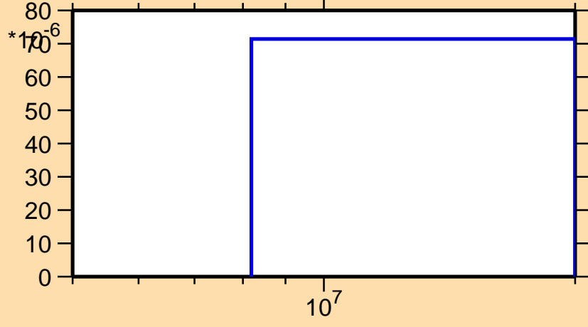
\sigma vs. E for ^{137}\text{Pr}(n,t)
