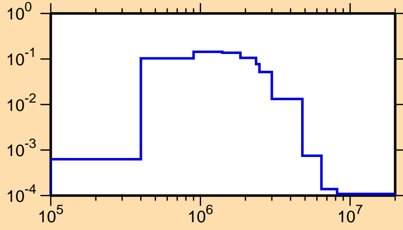
\sigma vs. E for ^{137}\text{Pr}(n,n_4)
