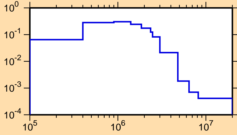
\sigma vs. E for ^{137}\text{Pr}(n,n_2)
