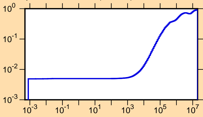
\mu vs. E for ^{138}\text{Pr}(\text{mt251})
