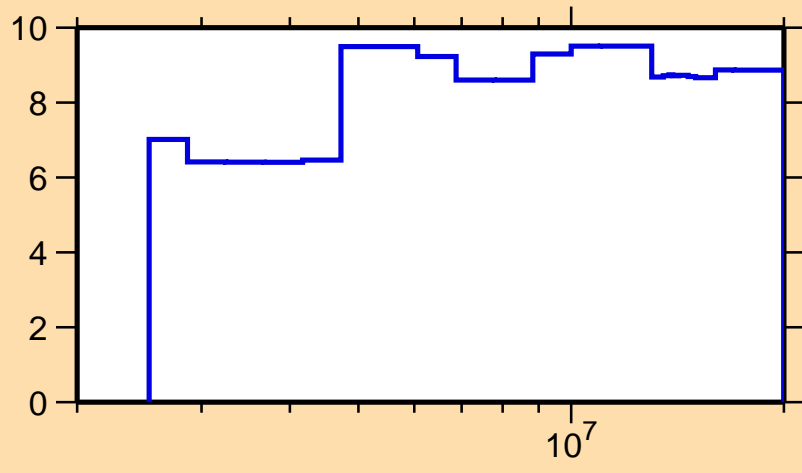
\Delta\sigma/\sigma vs. E for ^{138}\text{Pr}(n,\text{nonel.})
