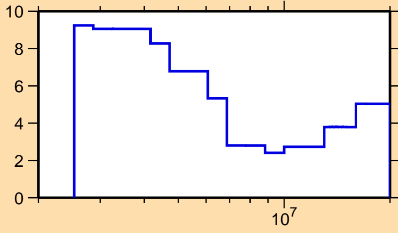
\Delta\sigma/\sigma vs. E for ^{138}\text{Pr}(n,\text{tot.})
