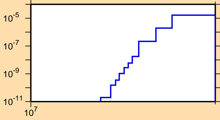
\sigma vs. E for ^{138}\text{Pr}(n,2n\alpha)
