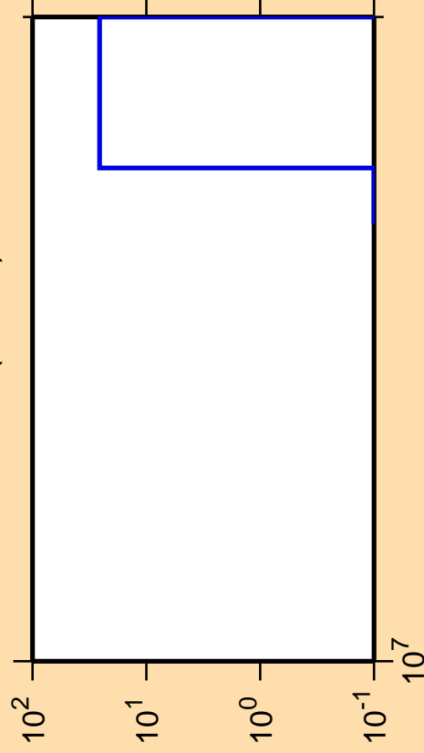
\Delta\sigma/\sigma vs. E for ^{138}\text{Pr}(\text{mt 34})
