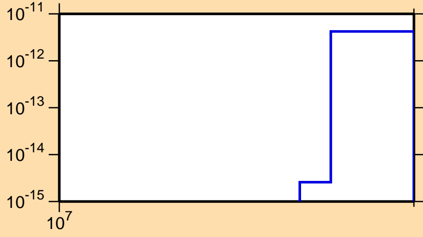
\sigma vs. E for ^{138}\text{Pr}(\text{mt 34})
