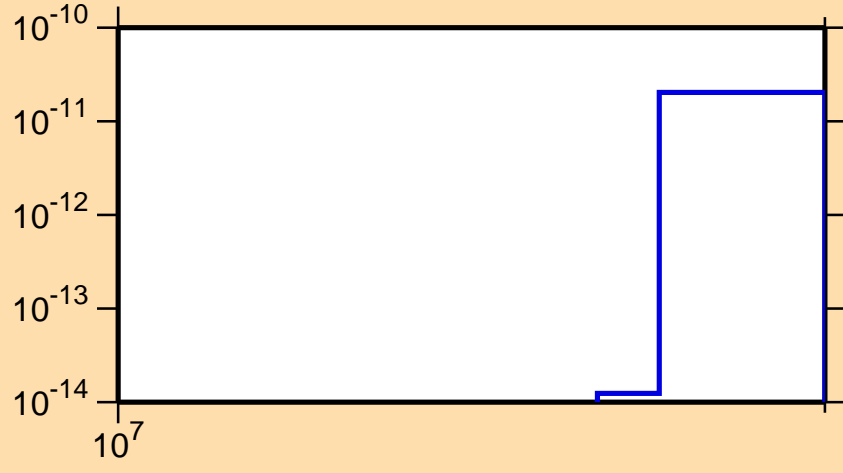
\sigma vs. E for ^{138}\text{Pr}(n,\text{pt})
