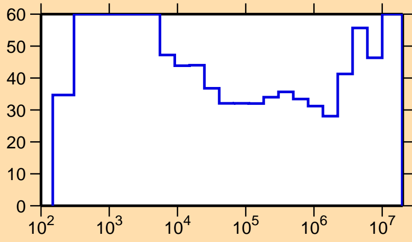
\Delta\sigma/\sigma vs. E for ^{138}\text{Pr}(n,\gamma)
