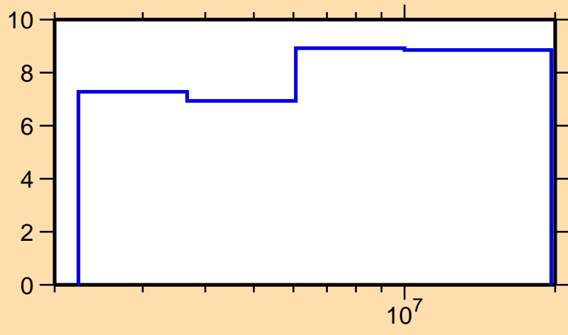
\Delta\sigma/\sigma vs. E for ^{138}\text{Pr}(n,n\text{onel.})
