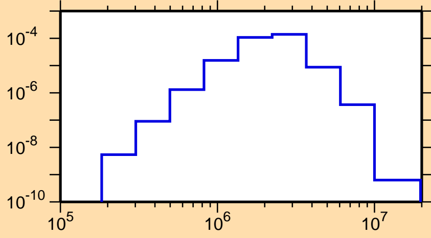
\sigma vs. E for ^{138}\text{Pr}(n,n_4)
