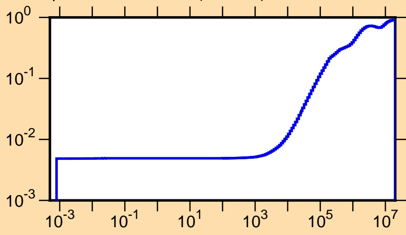
\mu vs. E for ^{139}\text{Pr}(\text{mt251})
