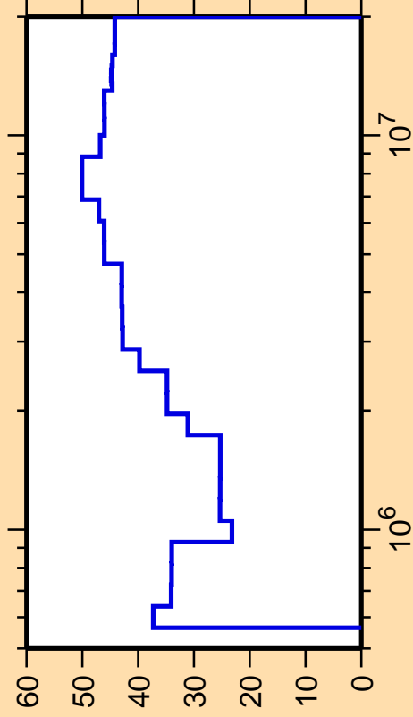
\Delta\sigma/\sigma vs. E for ^{139}\text{Pr}(n,n_3)
