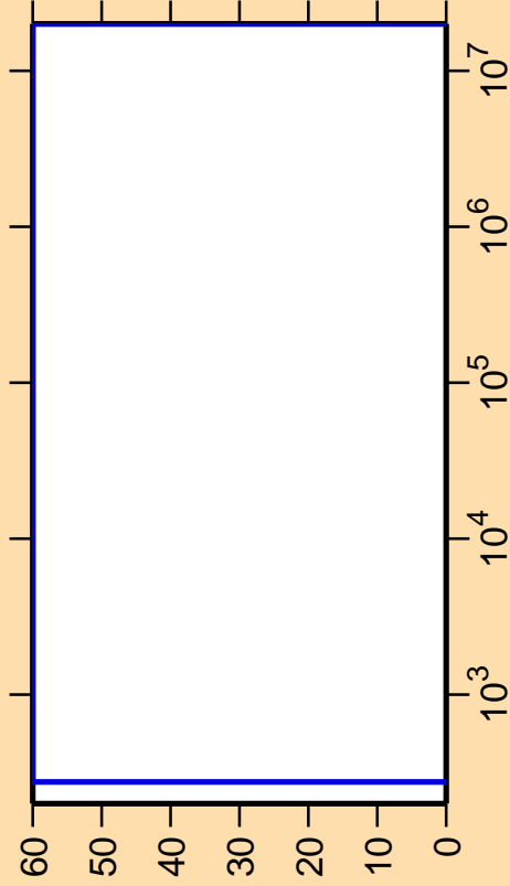
\Delta\sigma/\sigma vs. E for ^{139}\text{Pr}(n,\alpha)
