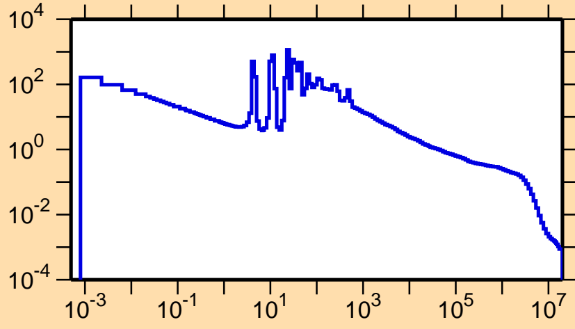
\sigma vs. E for ^{139}\text{Pr}(n,\gamma)
