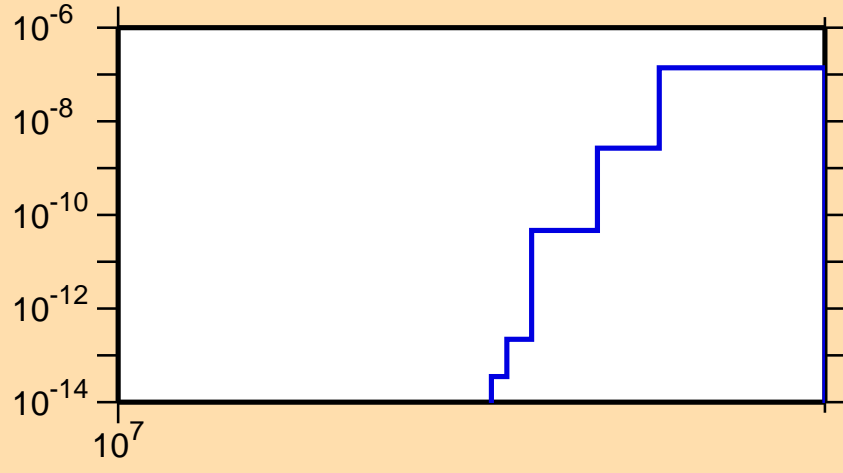
\sigma vs. E for ^{139}\text{Pr}(n,2n\alpha)
