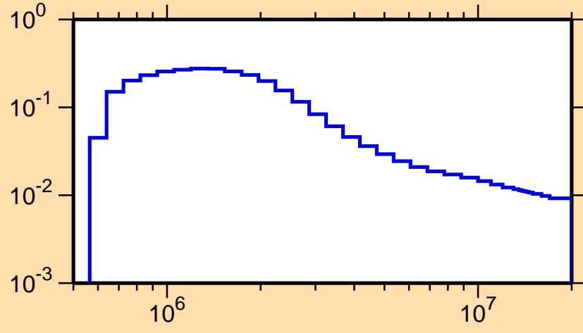
\sigma vs. E for ^{139}\text{Pr}(n,n_3)
