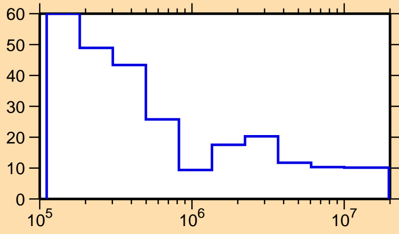
\Delta\sigma/\sigma vs. E for ^{139}\text{Pr}(n,\text{el.})
