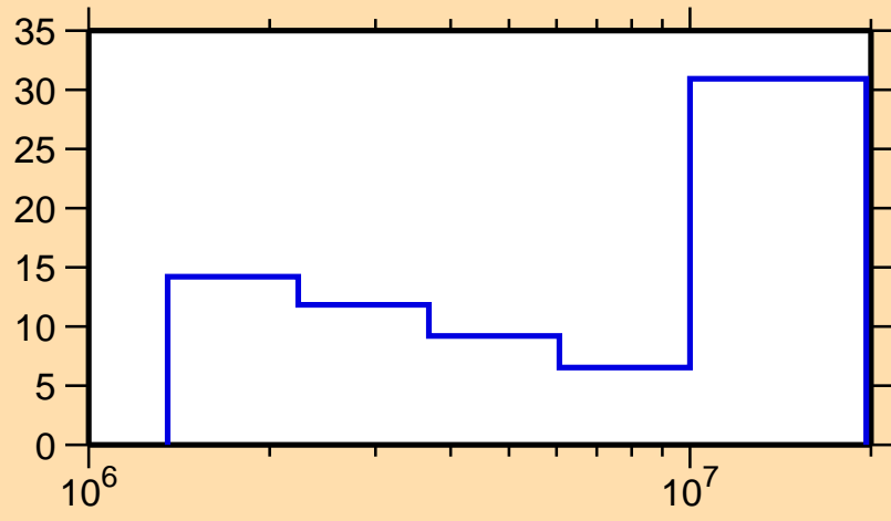
\Delta\sigma/\sigma vs. E for ^{139}\text{Pr}(n,\text{inel.})
