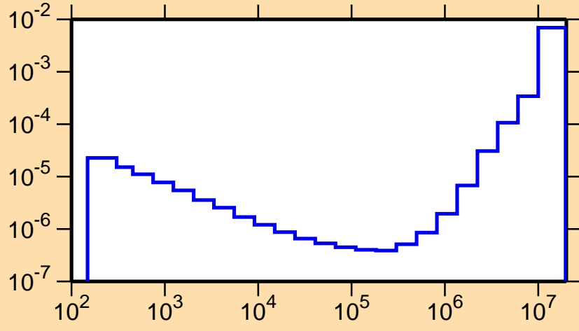
\sigma vs. E for ^{139}\text{Pr}(n,\alpha)
