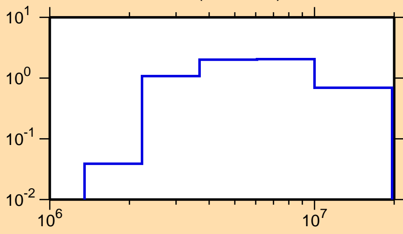
\sigma vs. E for ^{139}\text{Pr}(n,n\text{cont.})
