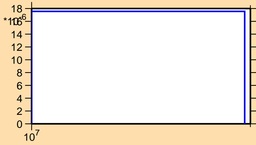
\sigma vs. E for ^{139}\text{Pr}(n,3n)
