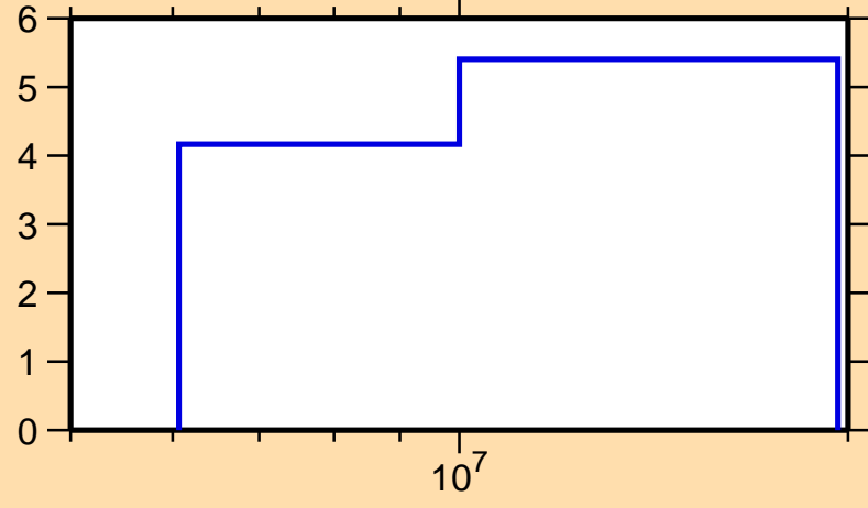
\Delta\sigma/\sigma vs. E for ^{139}\text{Pr}(n,\text{tot.})
