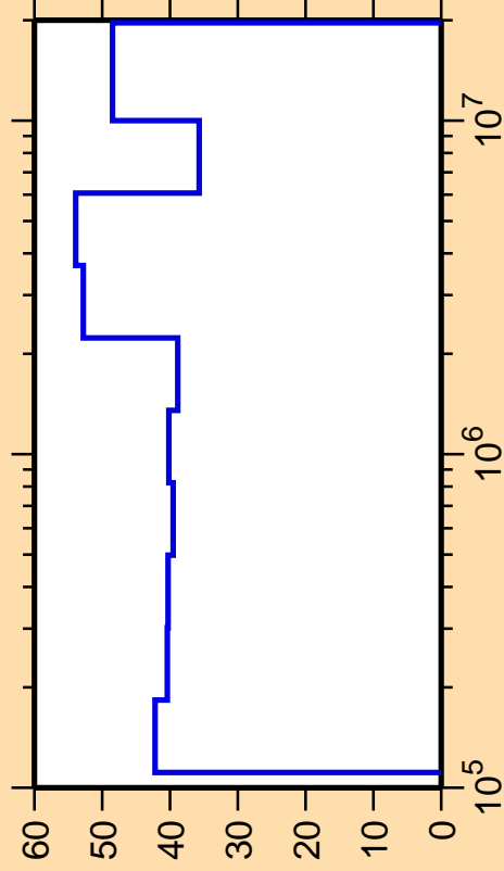
\Delta\sigma/\sigma vs. E for ^{139}\text{Pr}(n,p)
