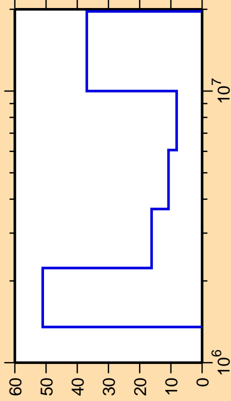
\Delta\sigma/\sigma vs. E for ^{139}\text{Pr}(n,n\text{cont.})
