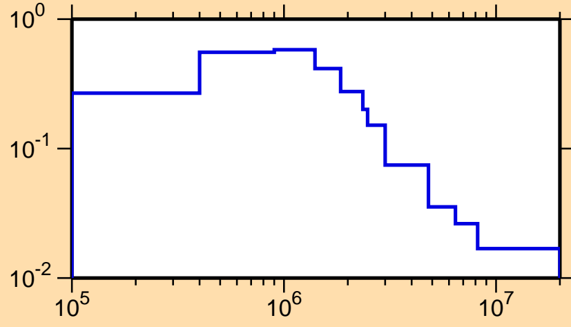
\sigma vs. E for ^{139}\text{Pr}(n,n_1)
