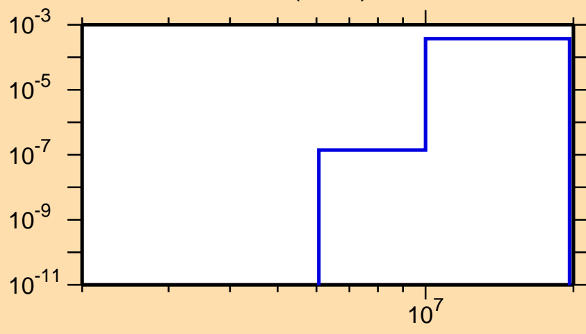
\sigma vs. E for ^{140}\text{Pr}(n,n\alpha)
