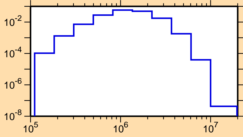
\sigma vs. E for ^{140}\text{Pr}(n,n_3)
