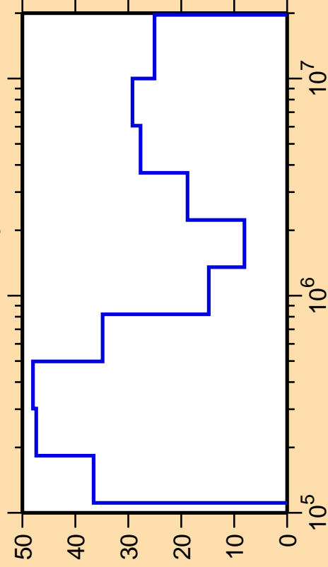
\Delta\sigma/\sigma vs. E for ^{140}\text{Pr}(n,n_3)
