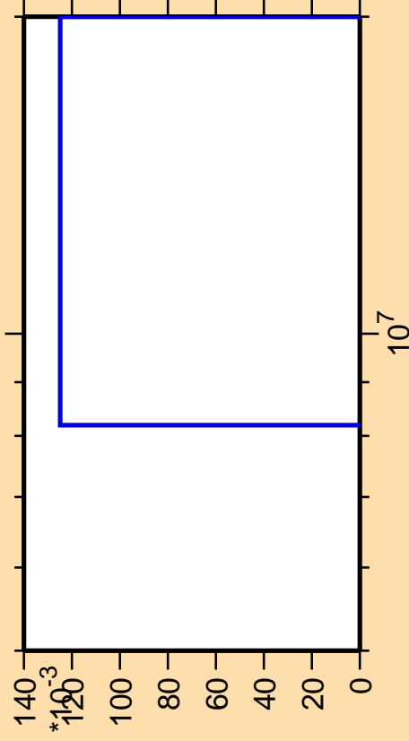
\Delta\sigma/\sigma vs. E for ^{140}\text{Pr}(\text{mt } 45)
