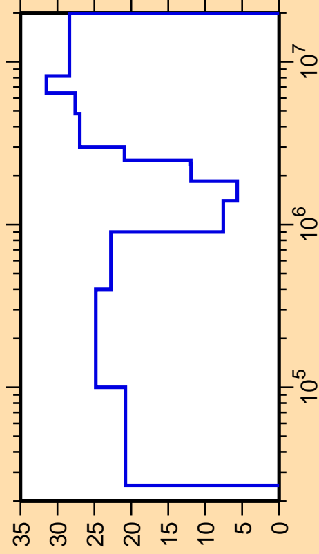
\Delta\sigma/\sigma vs. E for ^{140}\text{Pr}(n,n_2)
