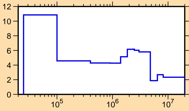
\Delta\sigma/\sigma vs. E for ^{140}\text{Pr}(n,\text{el.})
