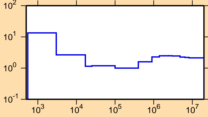
\sigma vs. E for ^{140}\text{Pr}(n,\text{nonel.})
