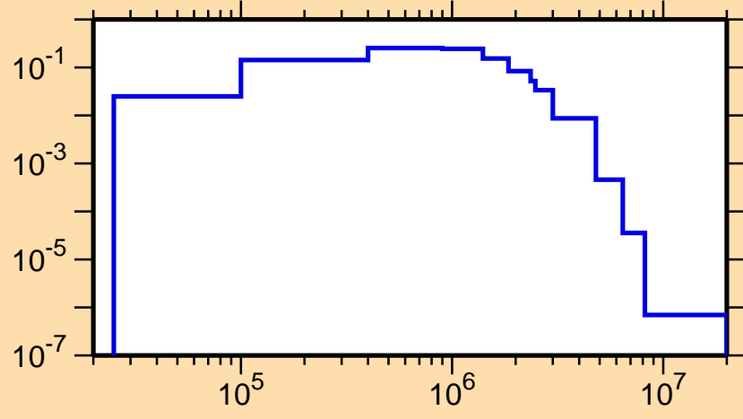
\sigma vs. E for ^{140}\text{Pr}(n,n_2)
