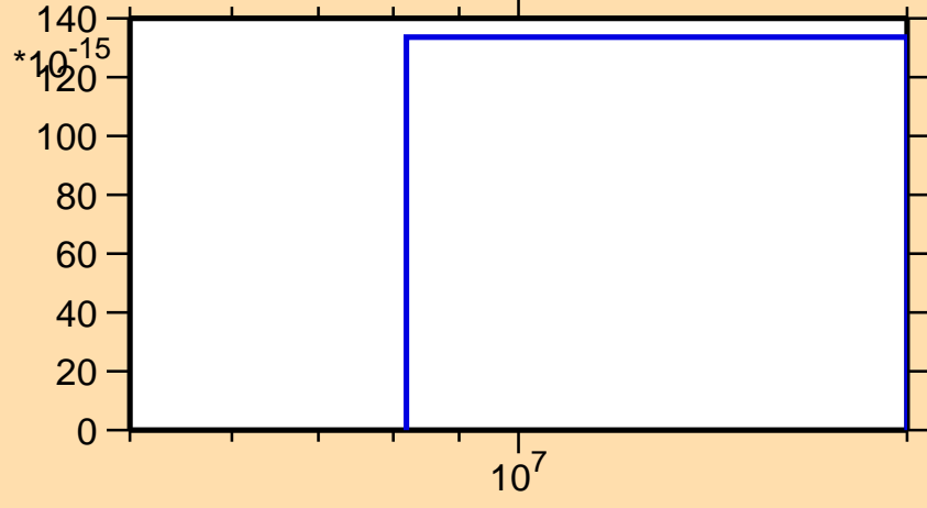
\sigma vs. E for ^{140}\text{Pr}(\text{mt } 45)
