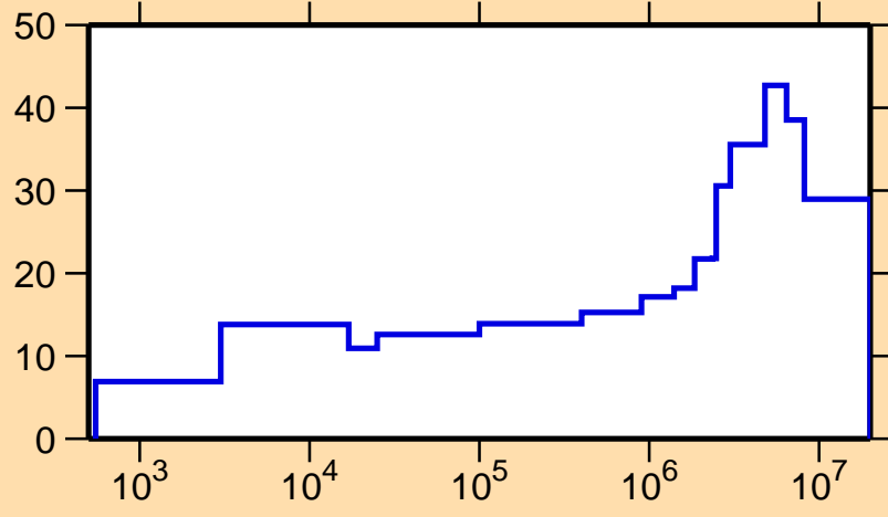
\Delta\sigma/\sigma vs. E for ^{140}\text{Pr}(n,\gamma)
