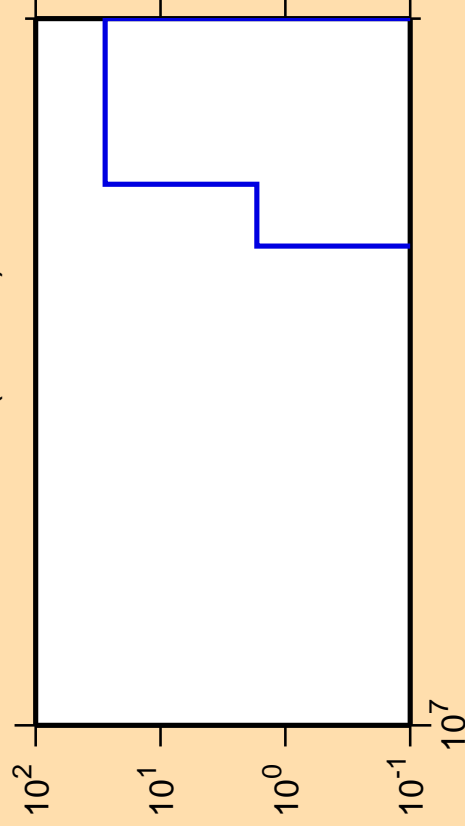
\Delta\sigma/\sigma vs. E for ^{141}\text{Pr}(\text{mt117})
