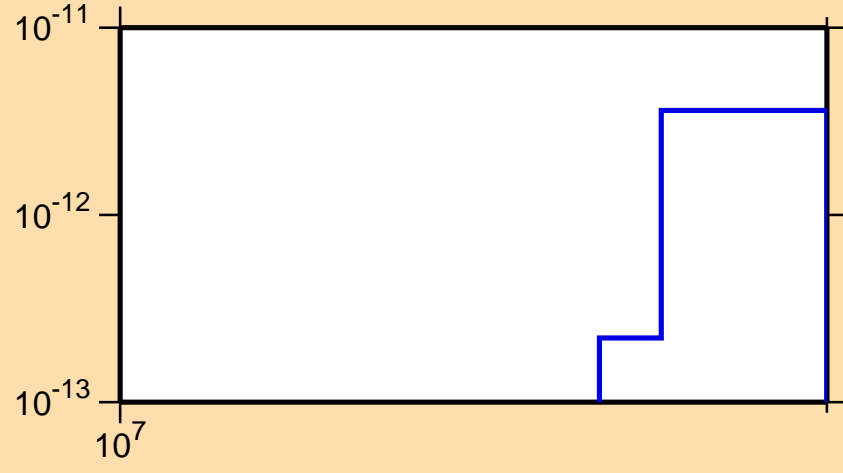
\sigma vs. E for ^{141}\text{Pr}(\text{mt117})
